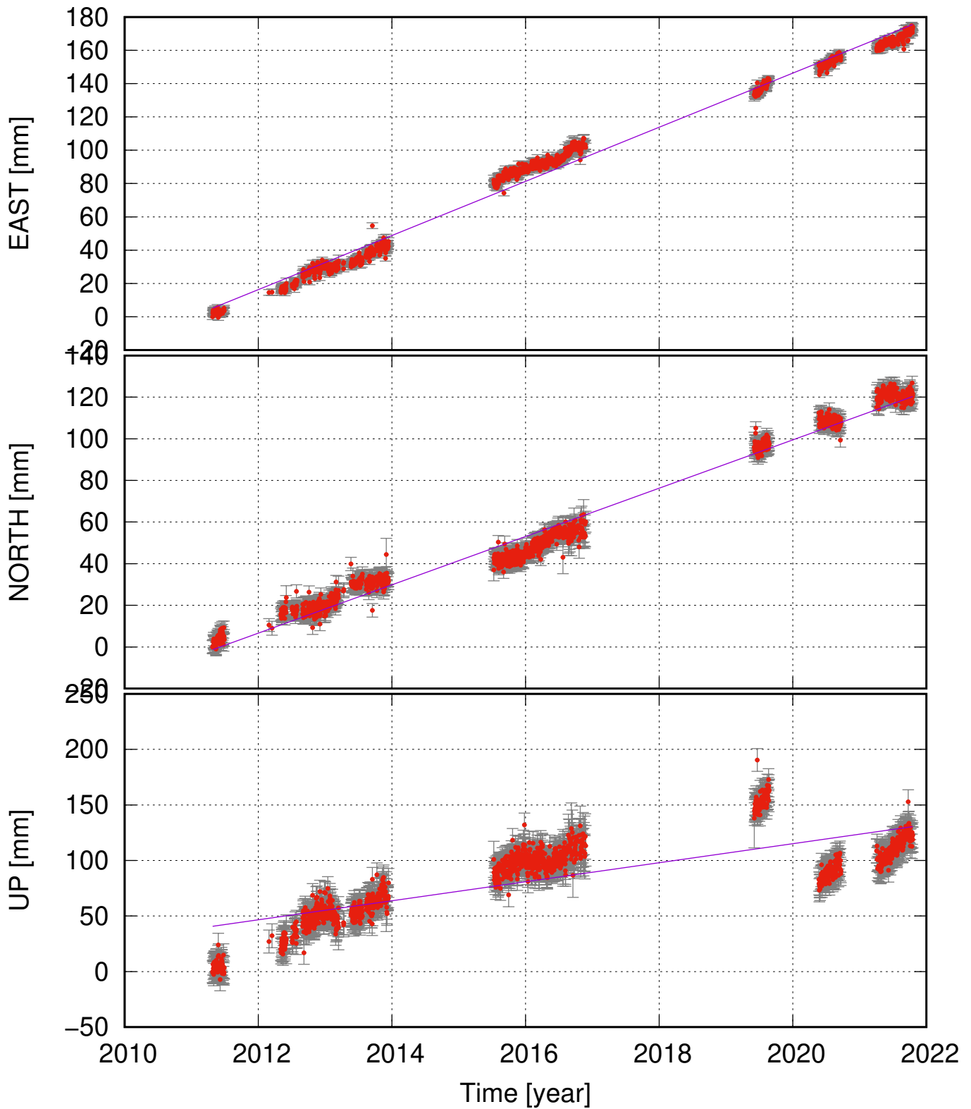
EYVI (64.23, -15.80) time series (ITRF 2014) ve = 16.25 ± 0.53; vn = 11.60 ± 0.52; vu = 8.57 ± 2.11 mm/yr
