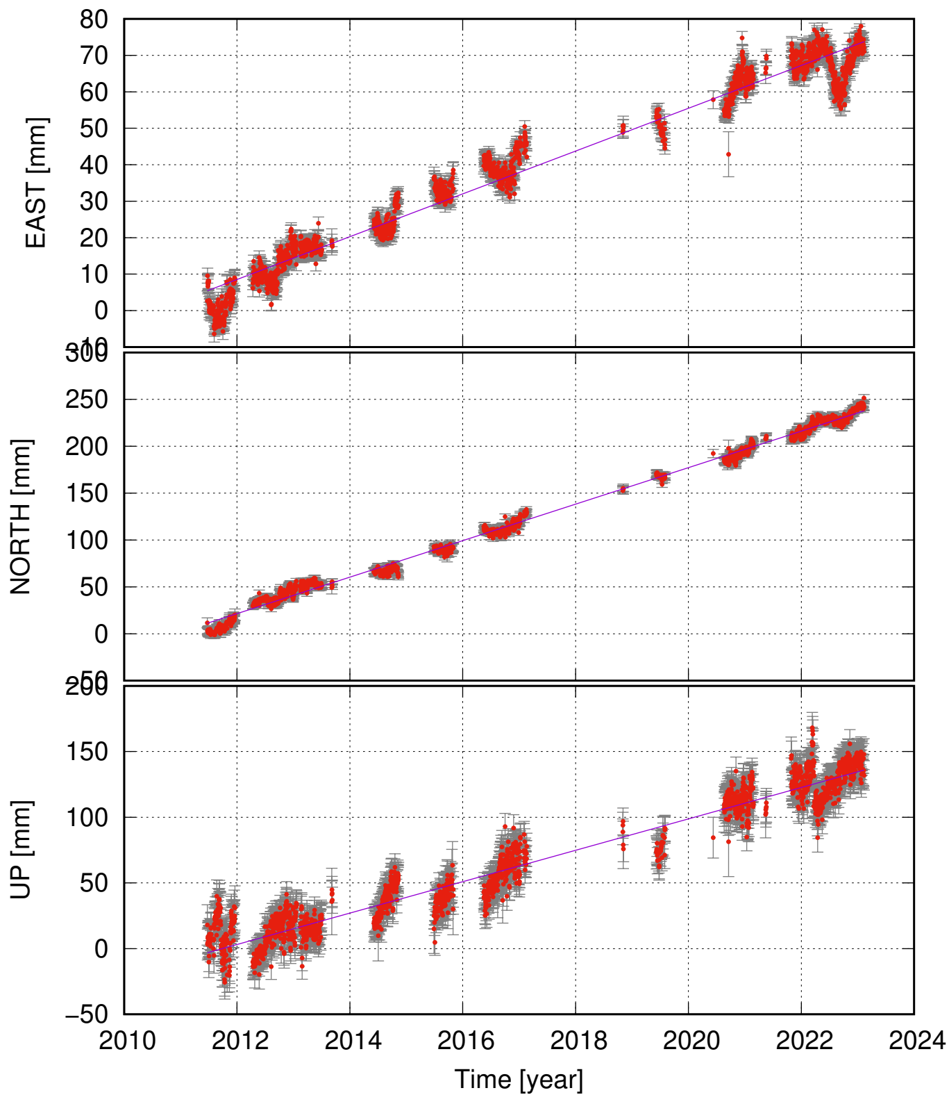
ENTC (63.70, -19.18) time series (ITRF 2014) v_e = 5.87 \pm 0.38 ; v_n = 19.45 \pm 0.48 ; v_u = 11.95 \pm 1.02 mm/yr
