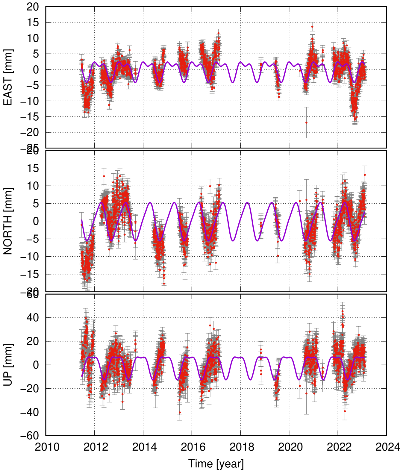
ENTC seasonal fit
