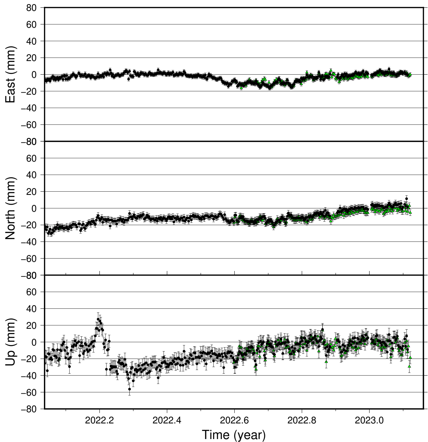
ENTC time series (IGS 2014), last 400 days
