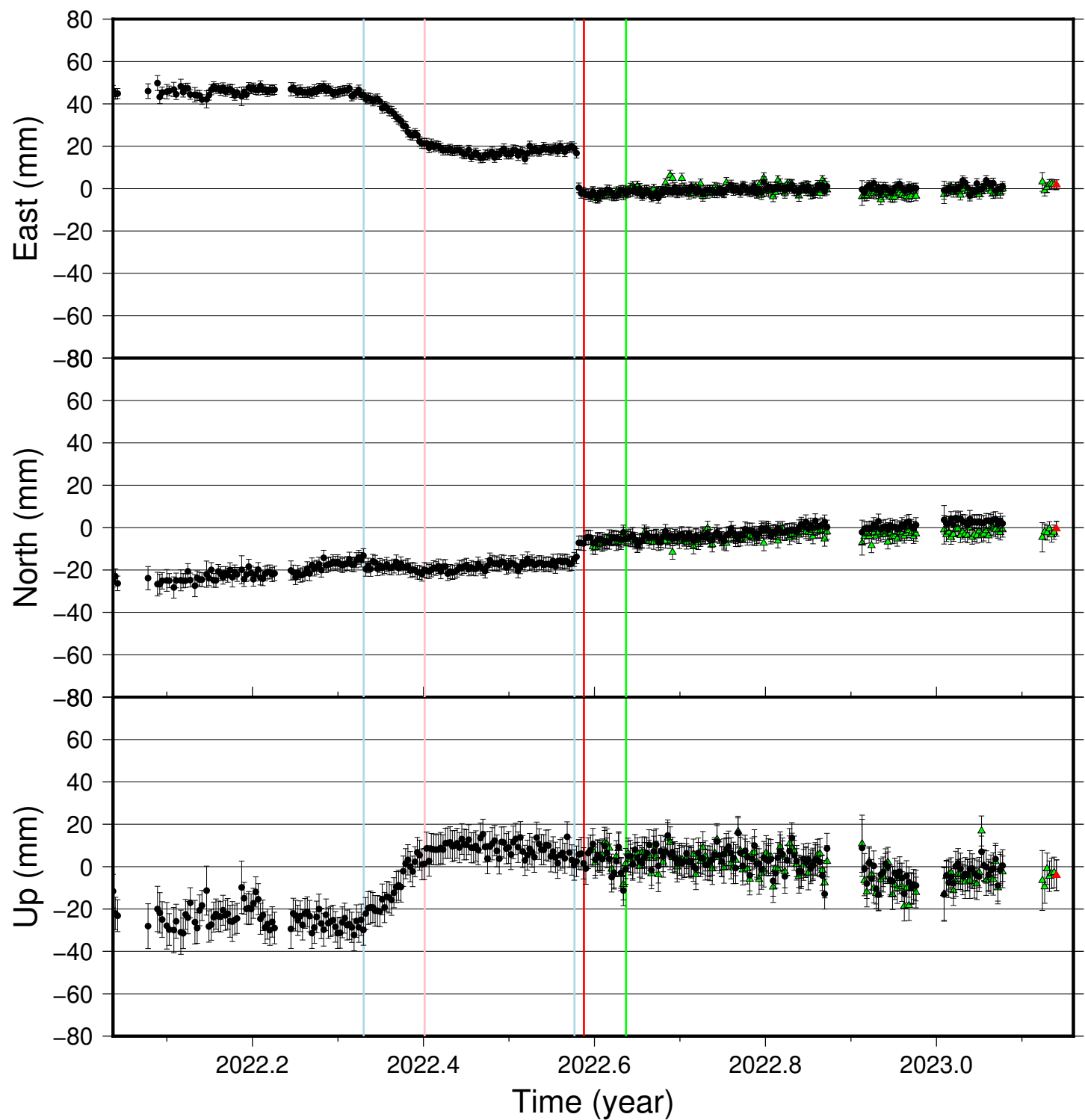
ELDC time series (IGS 2014), last 400 days
