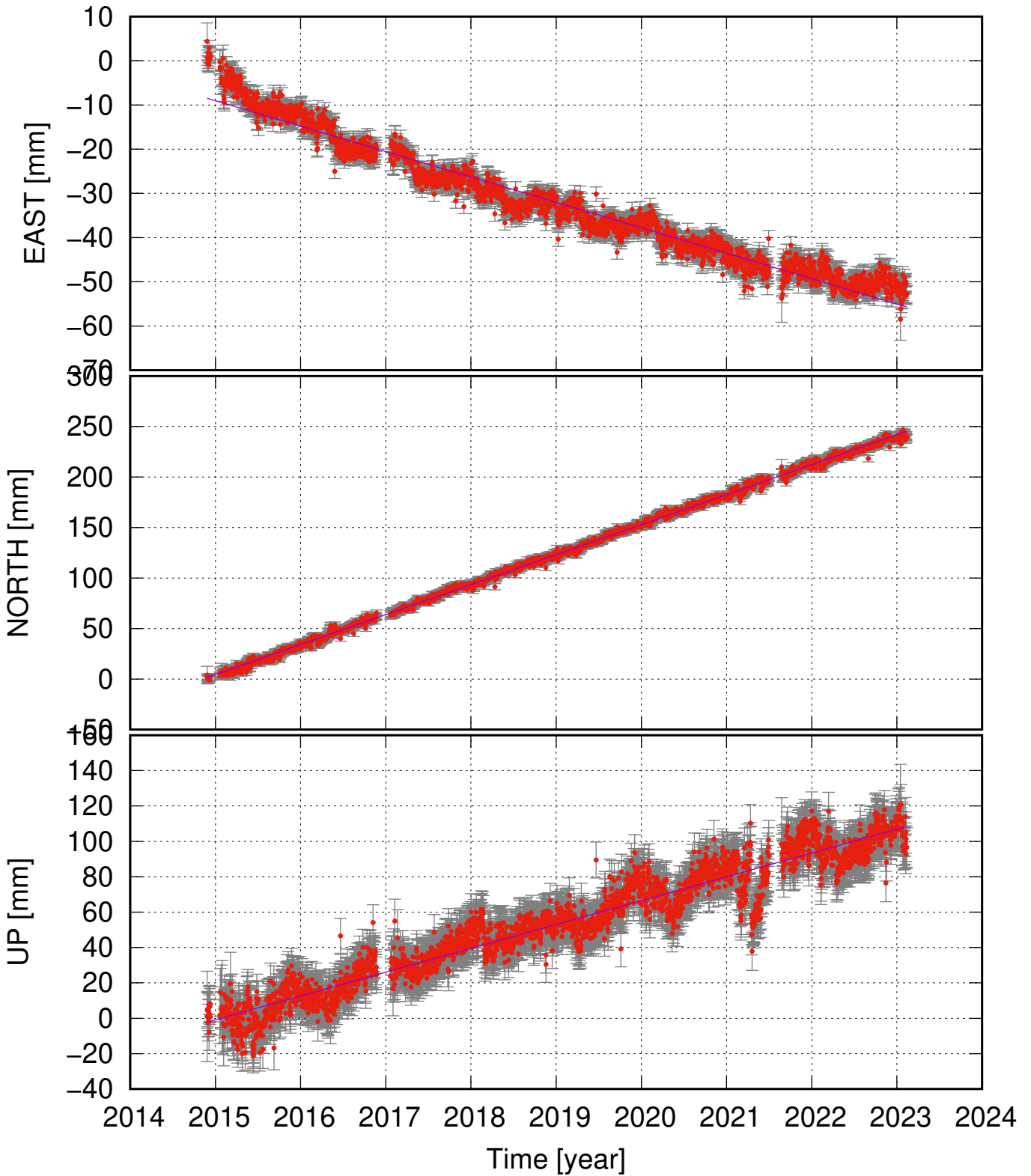
DYNY (65.02, -17.12) time series (ITRF 2014) v_e = -5.75 \pm 0.33 ; v_n = 29.68 \pm 0.29 ; v_u = 13.46 \pm 1.04 mm/yr
