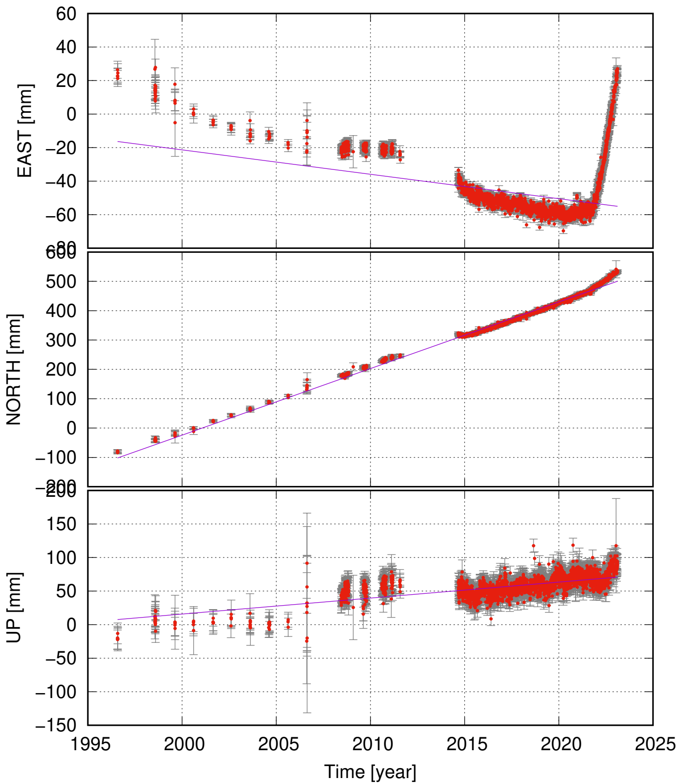
DYNG (65.06, -16.65) time series (ITRF 2014) v_e = -1.46 \pm 0.63 ; v_n = 22.72 \pm 0.35 ; v_u = 2.39 \pm 0.41 mm/yr
