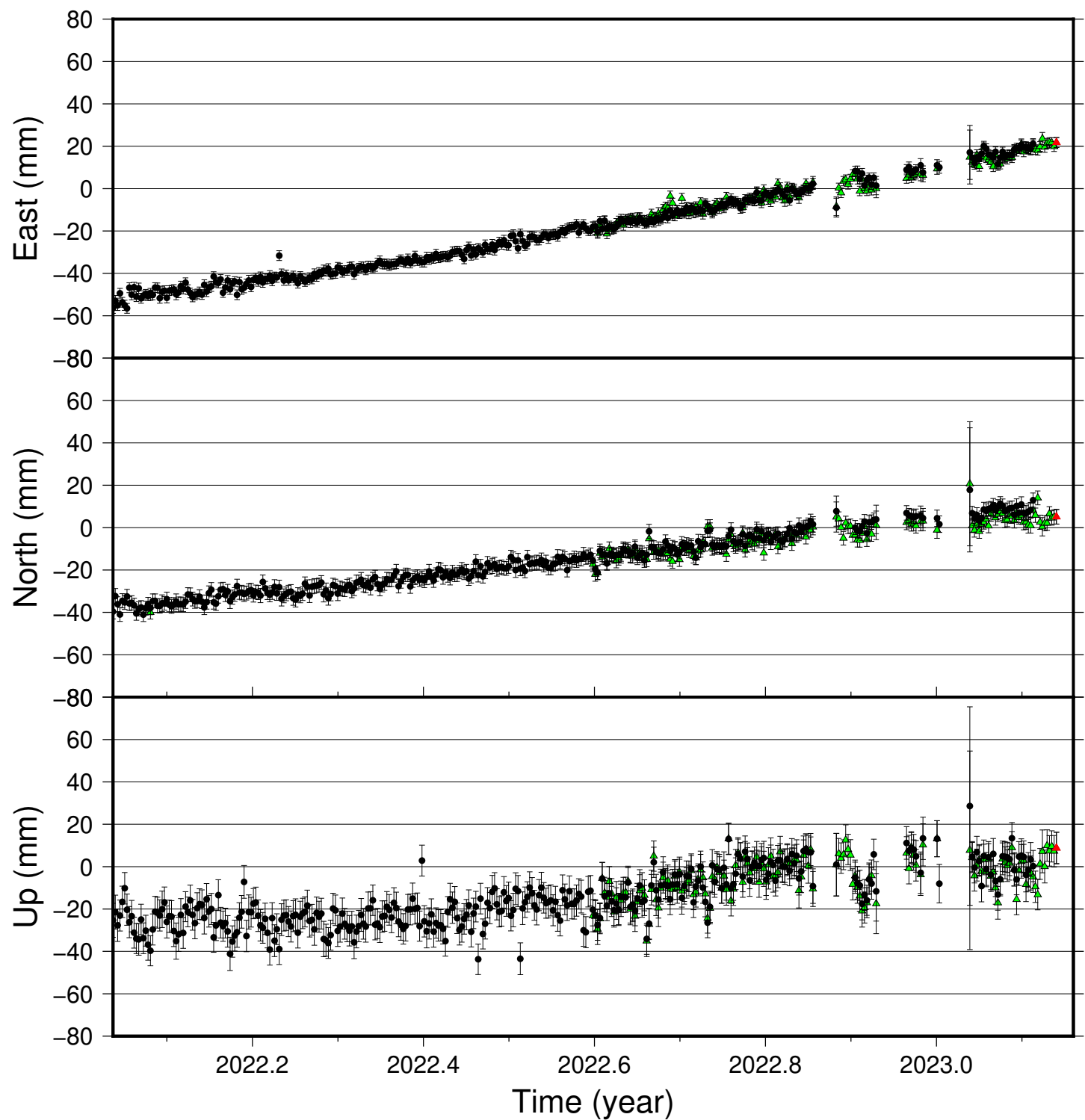
DYNG time series (IGS 2014), last 400 days
