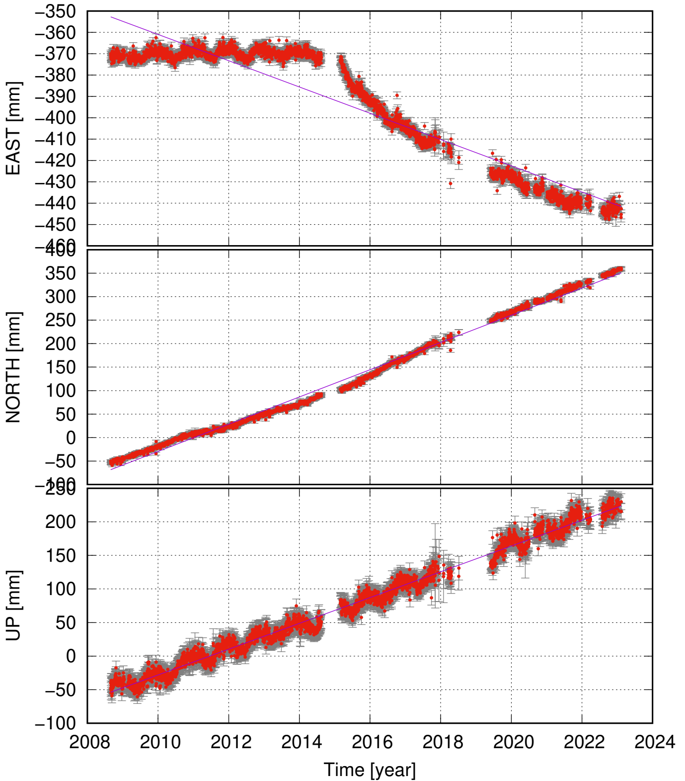
DYNC (64.79, -17.37) time series (ITRF 2014) v_e = -6.15 \pm 0.63 ; v_n = 28.99 \pm 0.70 ; v_u = 19.21 \pm 0.64 mm/yr
