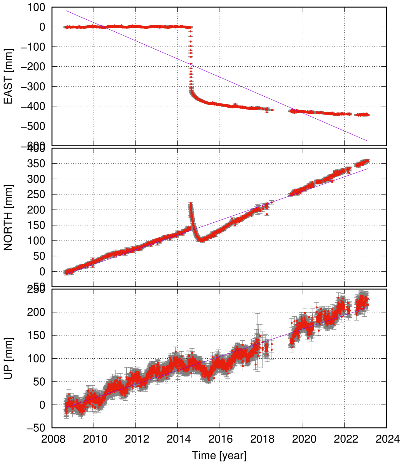
DYNC (64.79, -17.37) time series (ITRF 2014) ve = -45.58 \pm 6.91 ; vn = 23.68 \pm 1.24 ; vu = 14.96 \pm 0.94 mm/yr
