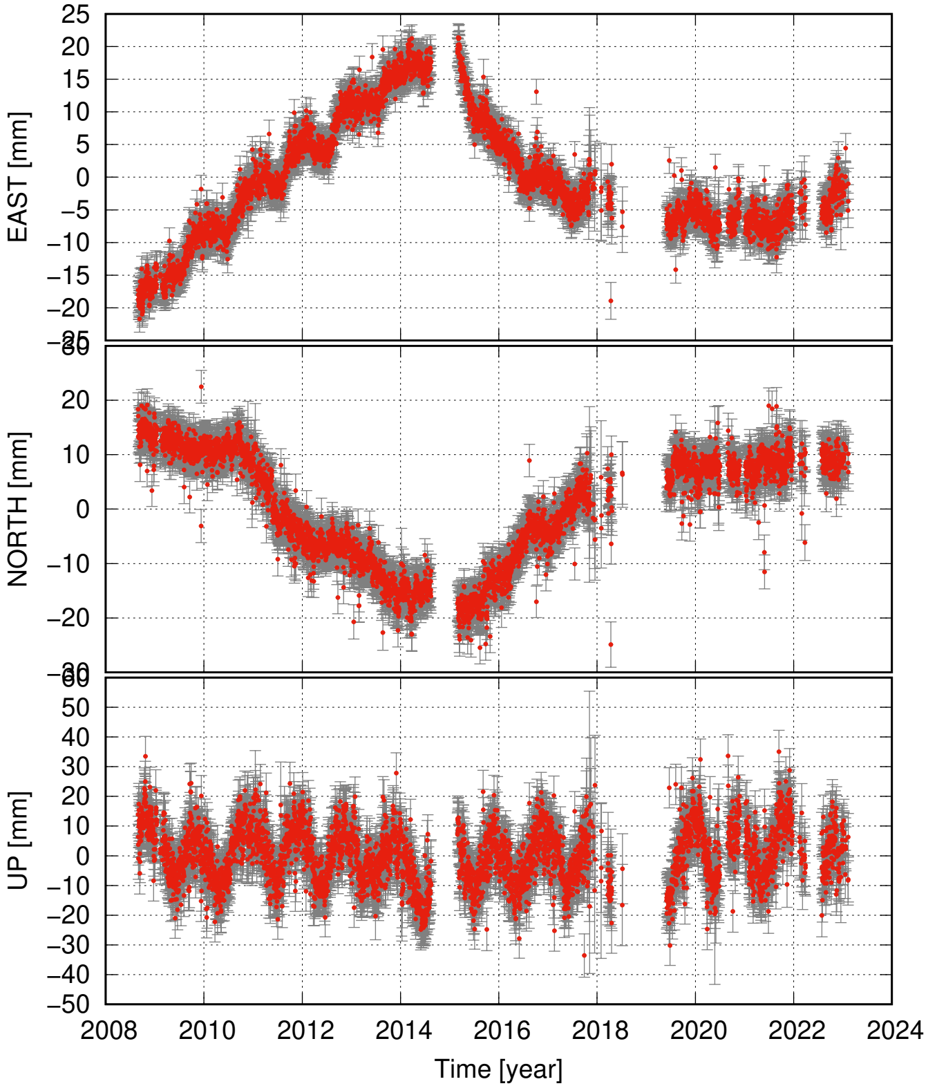
DYNC residual time series (some major events removed as well)
