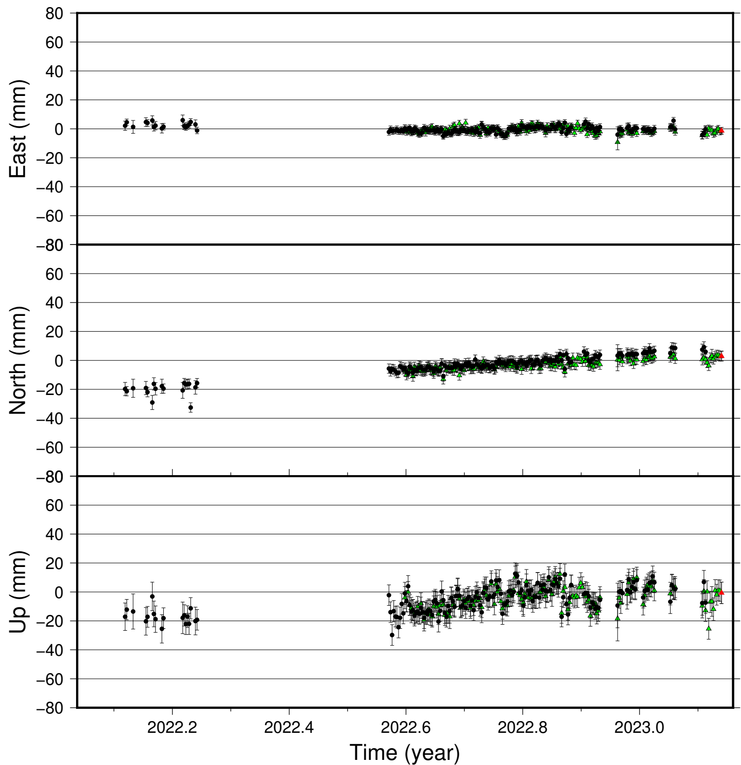
DYNC time series (IGS 2014), last 400 days
