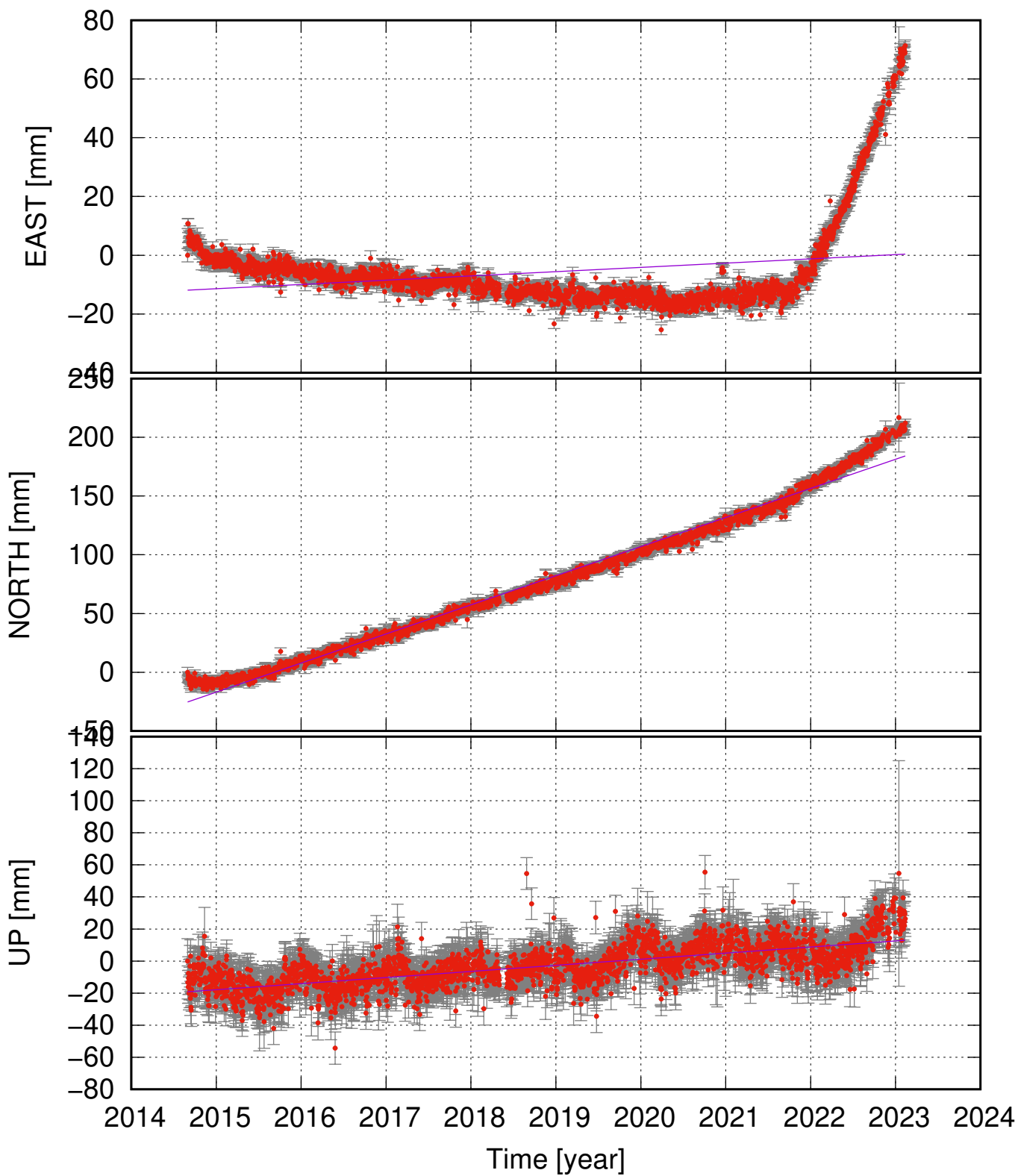
DYNA (65.06, -16.65) time series (ITRF 2014) v_e = 1.45 \pm 1.71 ; v_n = 24.77 \pm 0.83 ; v_u = 3.80 \pm 1.06 mm/yr
