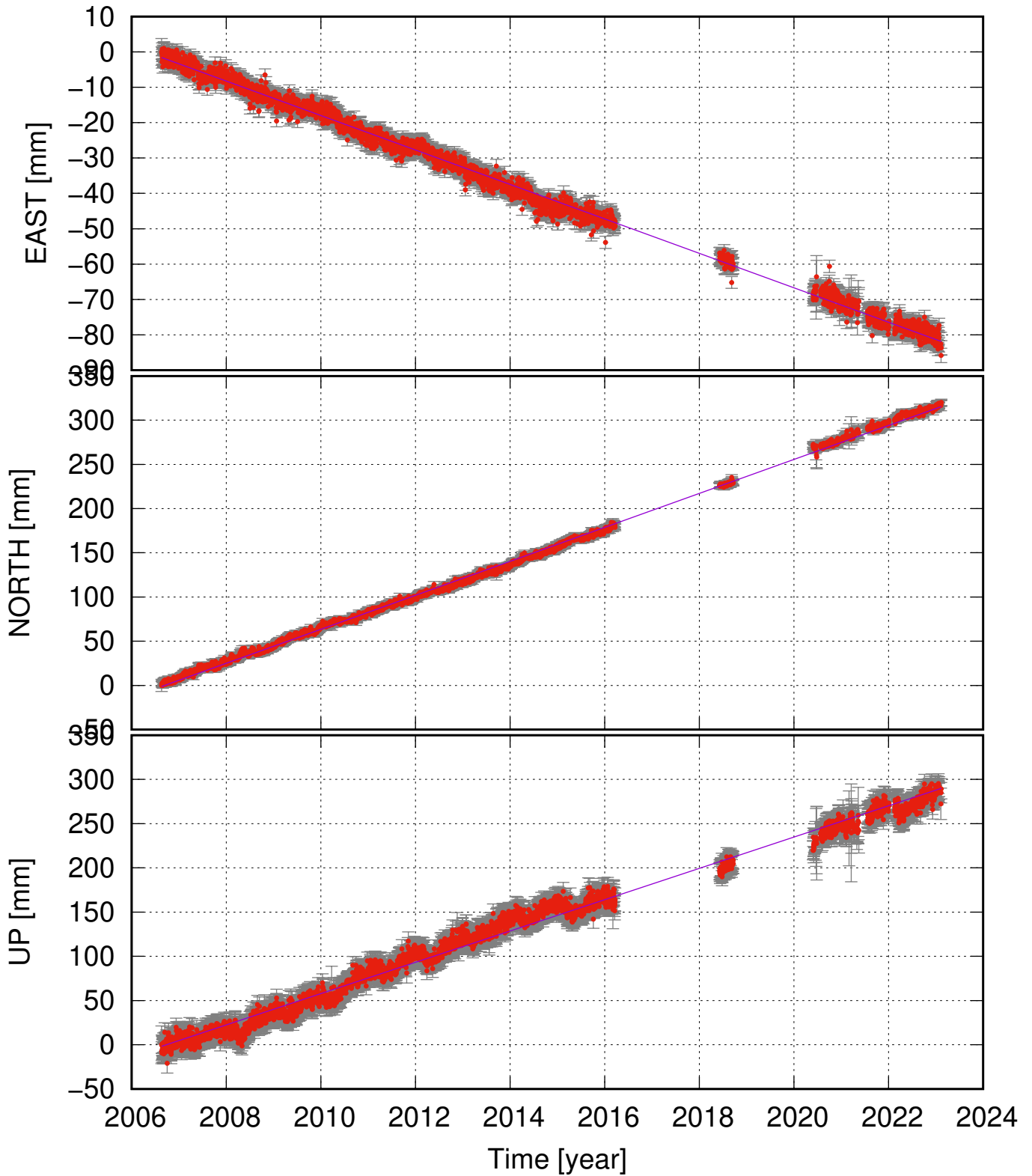
BUDH (64.24, -19.32) time series (ITRF 2014) v_e = -4.87 \pm 0.09 ; v_n = 19.22 \pm 0.20 ; v_u = 17.70 \pm 0.53 mm/yr
