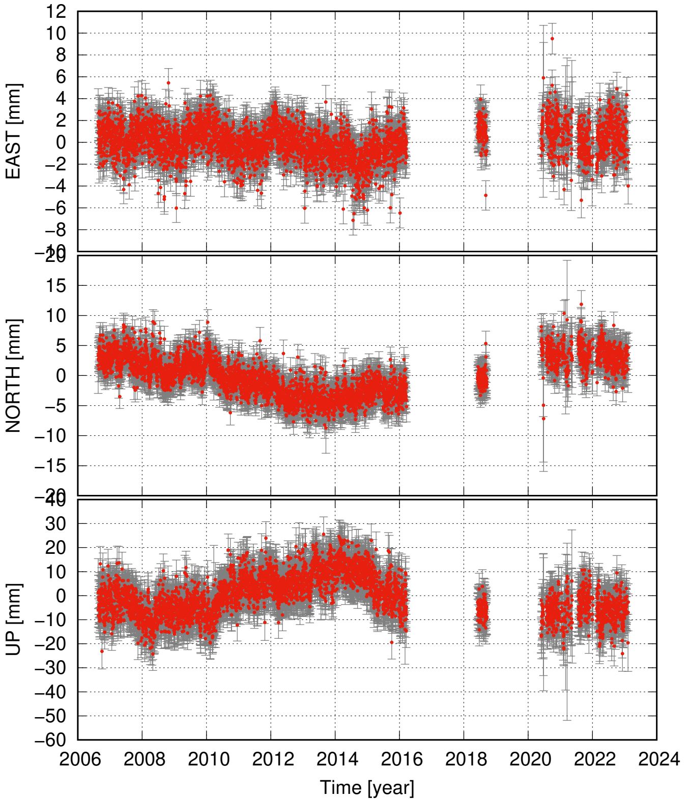
BUDH detrended and seasonal signal removed
