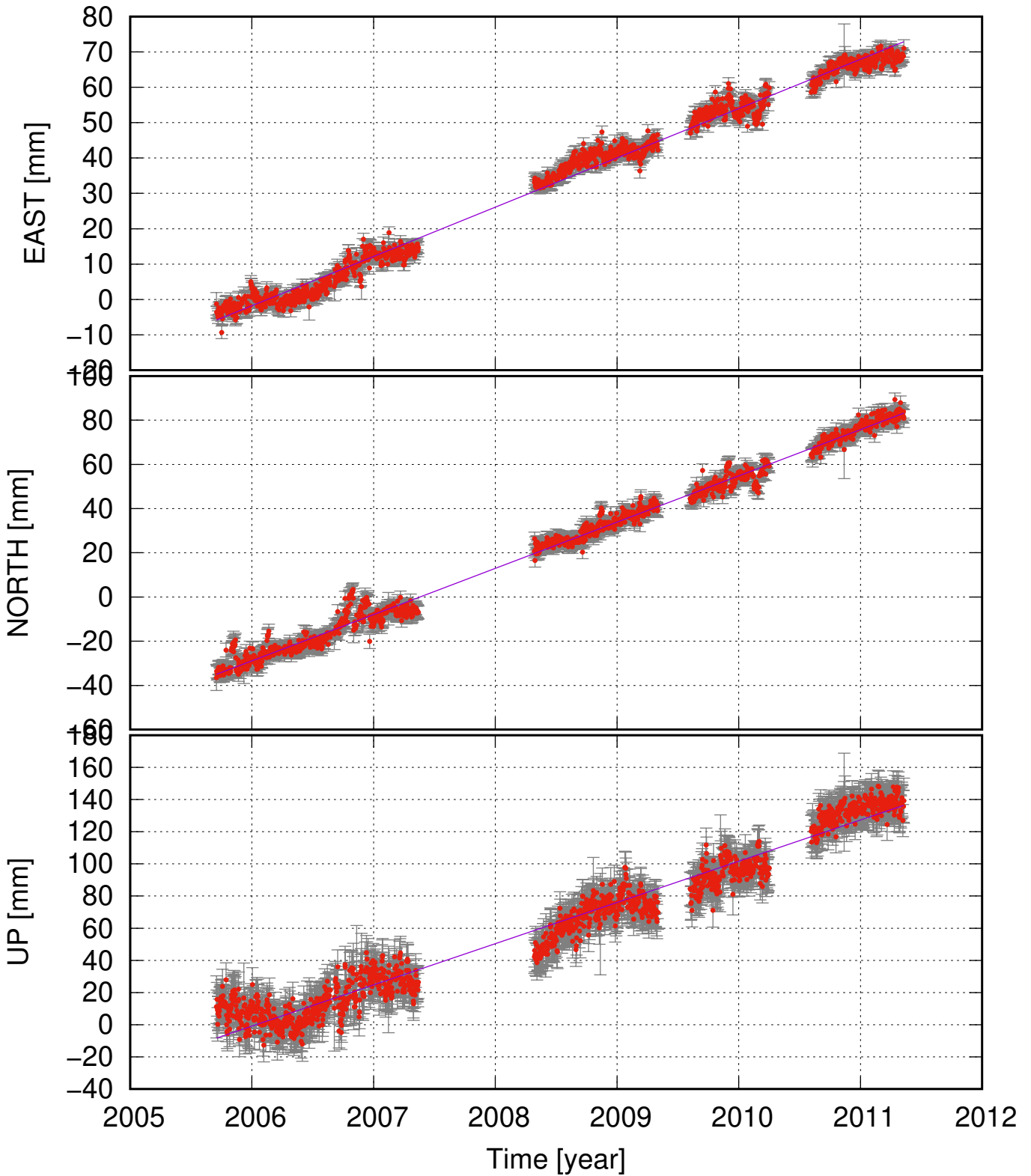
BRUJ (64.83, -16.09) time series (ITRF 2014) v_e = 13.94 \pm 0.45 ; v_n = 20.92 \pm 0.55 ; v_u = 25.64 \pm 1.62 mm/yr
