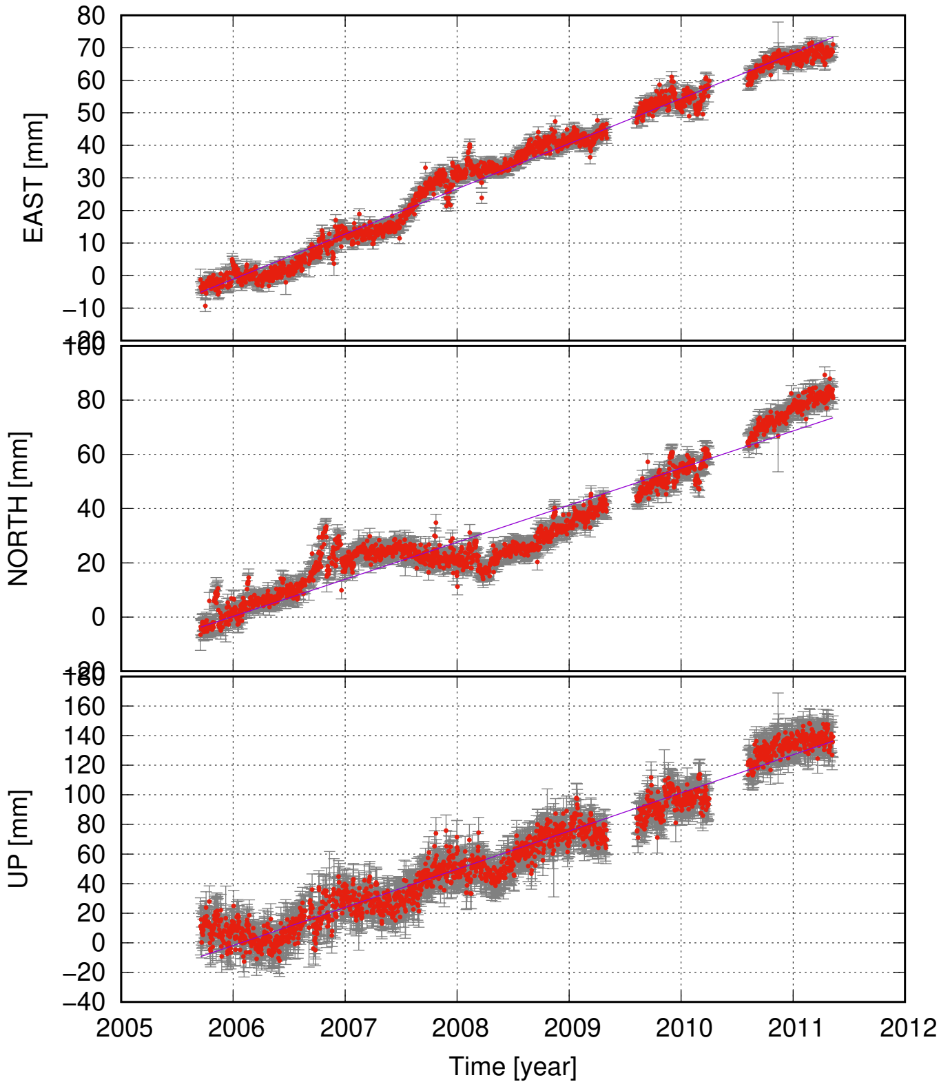
BRUJ (64.83, -16.09) time series (ITRF 2014) v_e = 13.87 \pm 0.53 ; v_n = 13.67 \pm 1.22 ; v_u = 25.78 \pm 1.60 mm/yr
