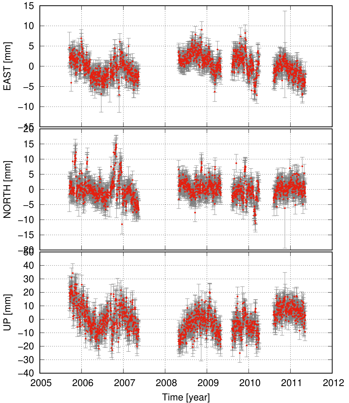
BRUJ residual time series (some major events removed as well)
