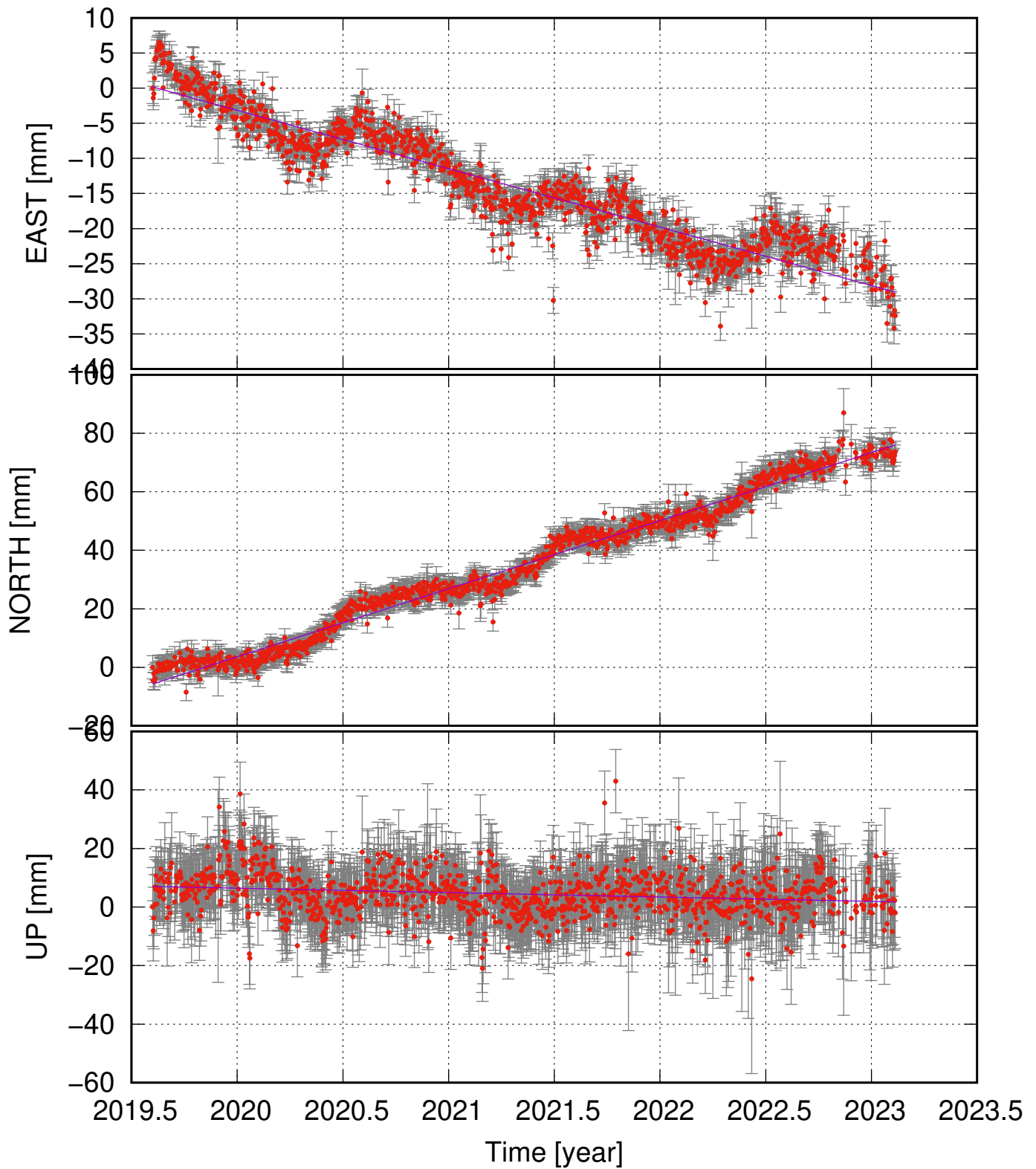
BRTT (66.12, -17.91) time series (ITRF 2014) v_e = -8.32 \pm 0.83 ; v_n = 23.27 \pm 0.96 ; v_u = -1.52 \pm 2.01 mm/yr
