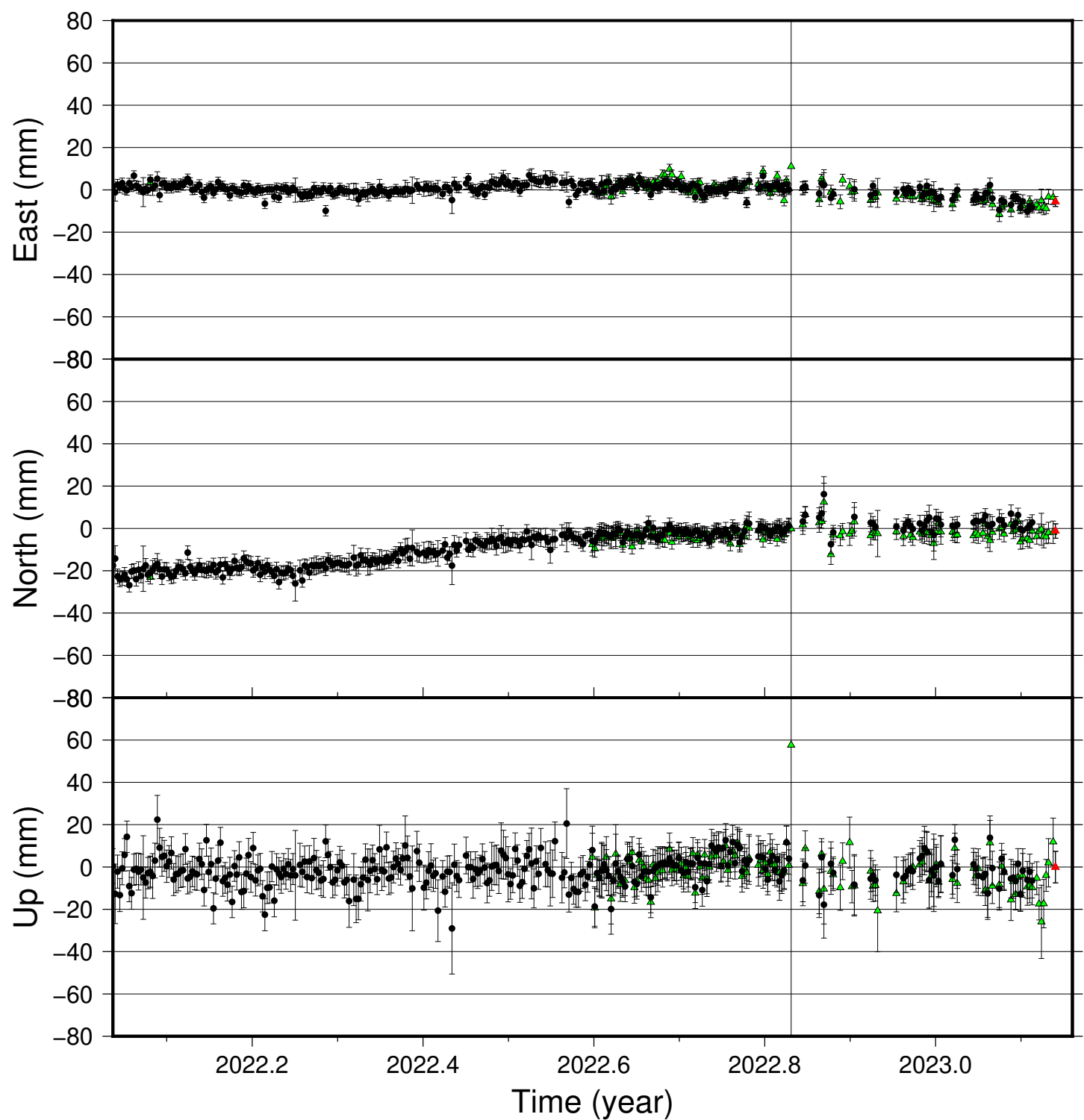
BRTT time series (IGS 2014), last 400 days
