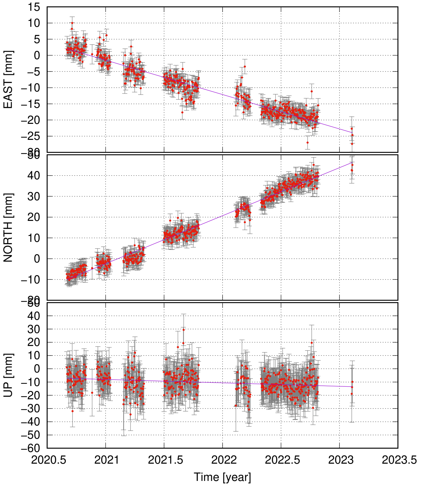
BRİK (66.12, -18.61) time series (ITRF 2014) v_e = -10.63 \pm 0.92 ; v_n = 23.10 \pm 1.00 ; v_u = -2.59 \pm 3.11 mm/yr
