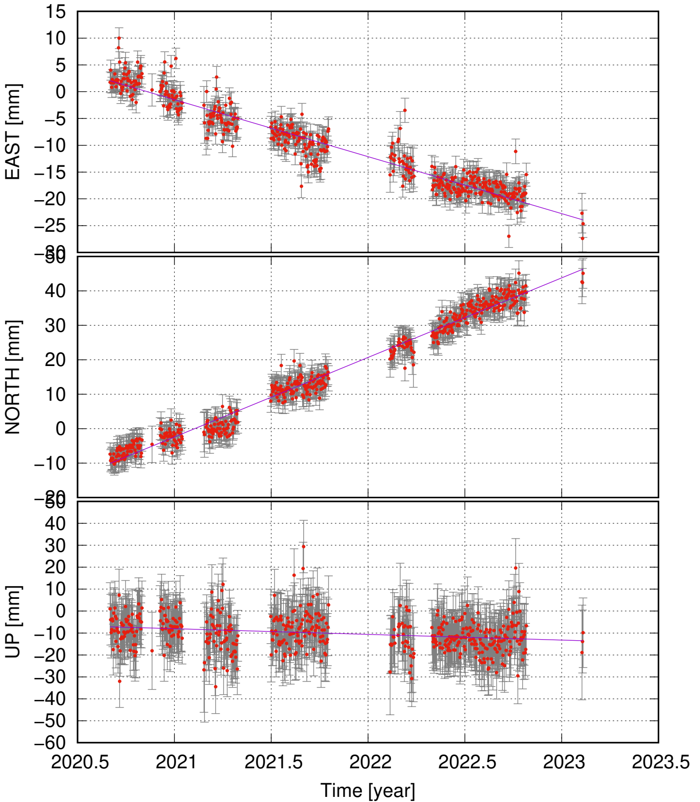
BR1K (66.12, -18.61) time series (ITRF 2014) v_e = -10.63 \pm 0.92 ; v_n = 23.10 \pm 1.00 ; v_u = -2.59 \pm 3.11 mm/yr
