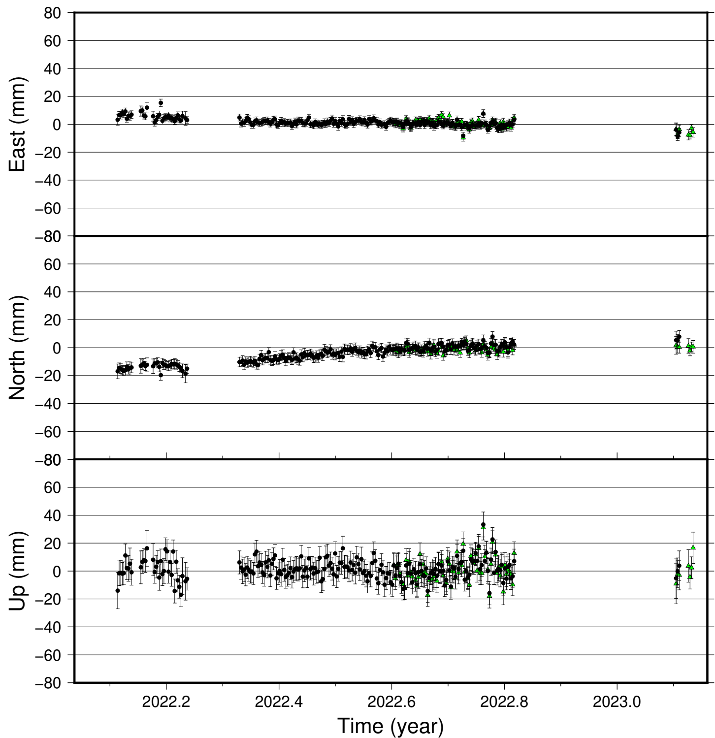
BRIC time series (IGS 2014), last 400 days
