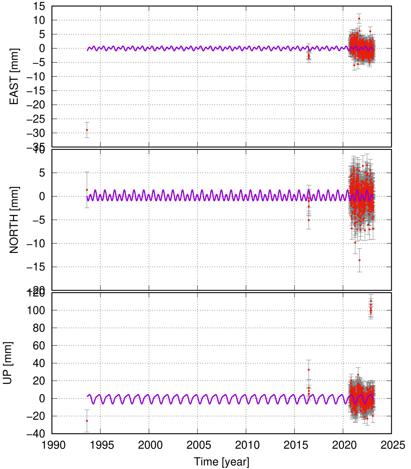
BLON seasonal fit
