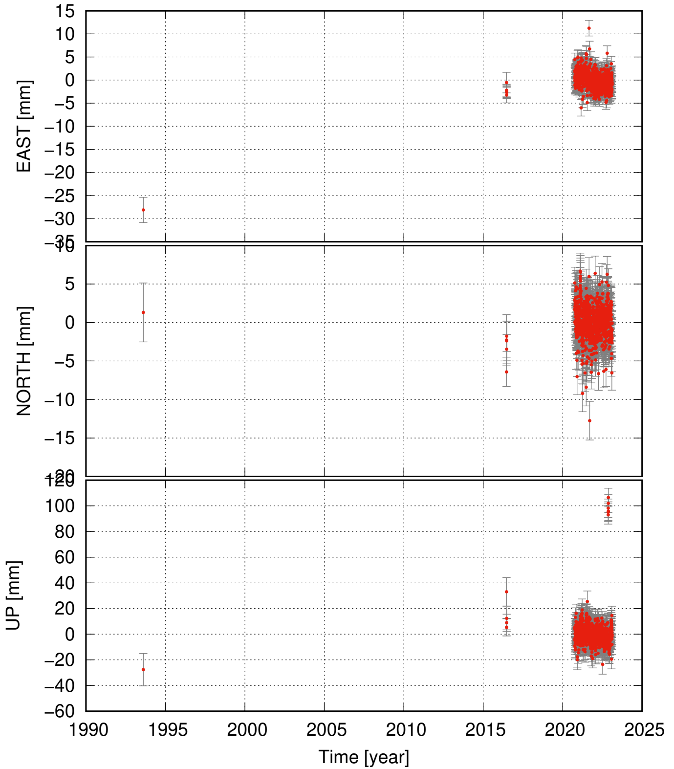
BLON detrended and seasonal signal removed
