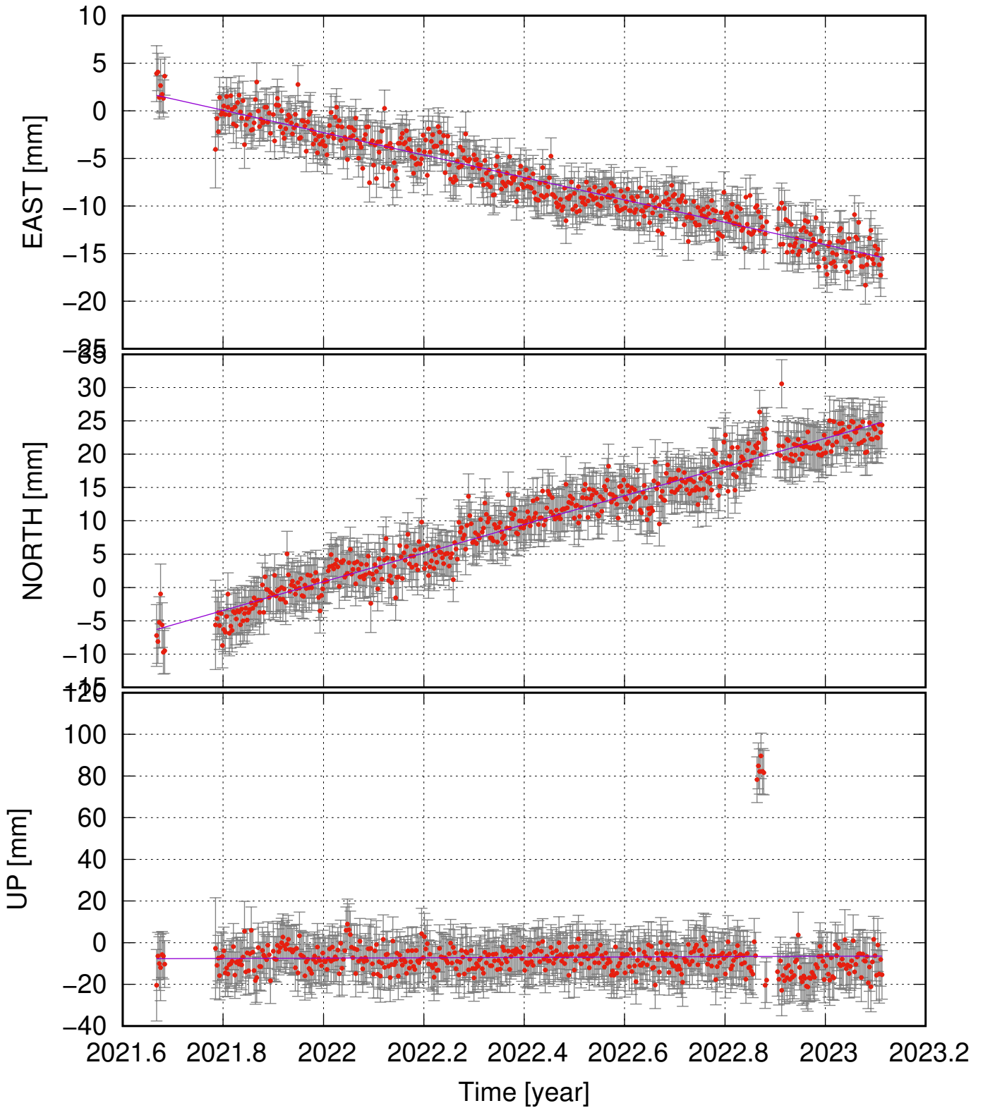
BJTV (65.50, -24.53) time series (ITRF 2014) v_e = -11.77 \pm 1.00 ; v_n = 21.52 \pm 1.39 ; v_u = 0.90 \pm 7.89 mm/yr
