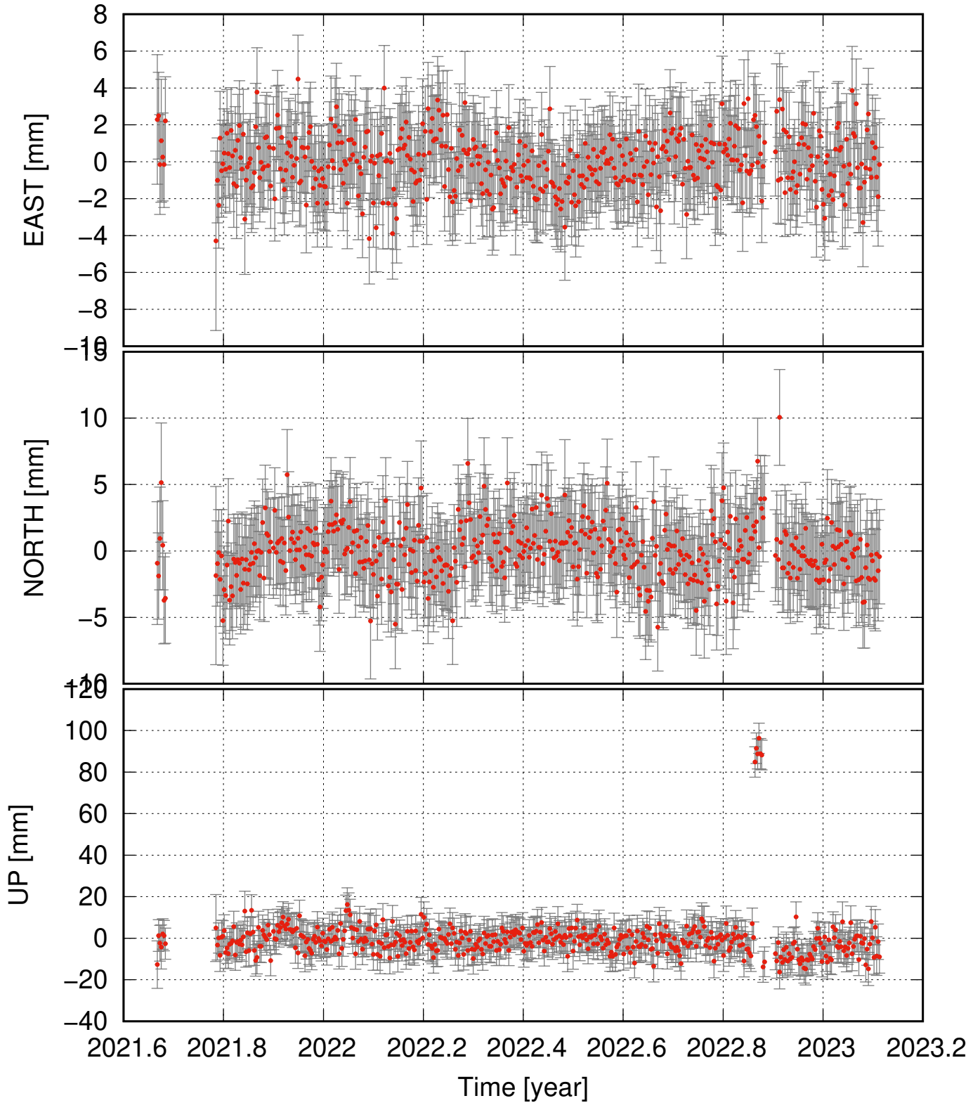
BJTV residual time series (some major events removed as well)
