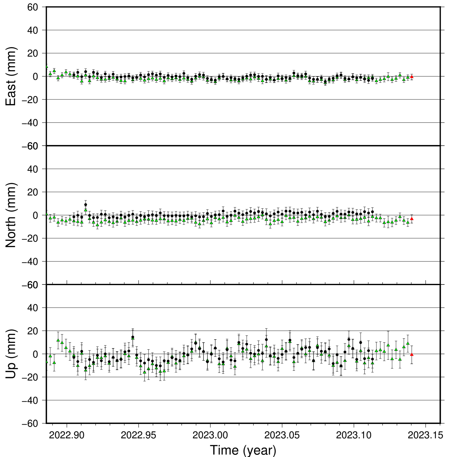
BJTV time series (IGS 2014), last 100 days
