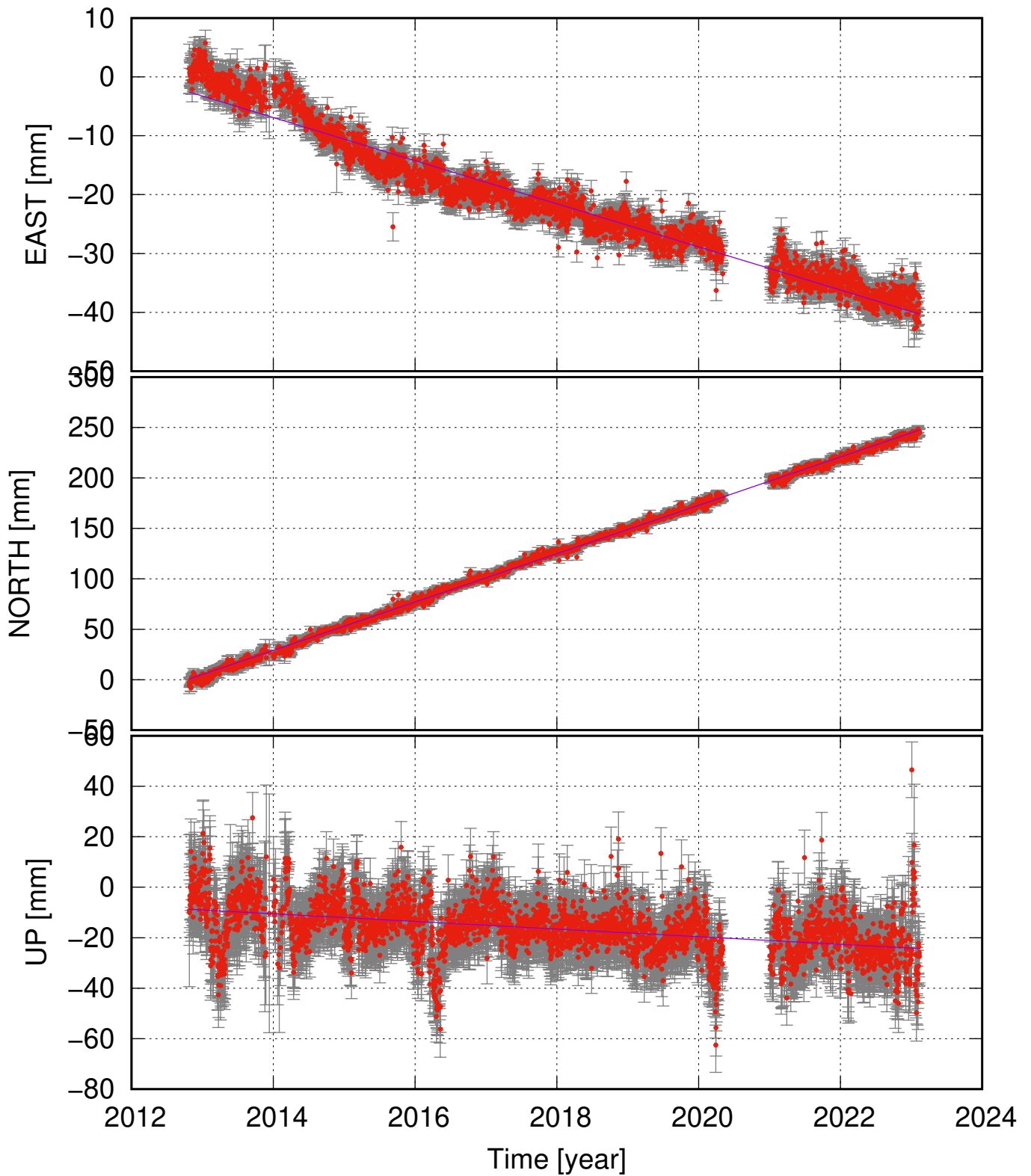
BJAC (65.61, -16.83) time series (ITRF 2014) v_e = -3.66 \pm 0.24 ; v_n = 23.96 \pm 0.27 ; v_u = -1.51 \pm 0.86 mm/yr
