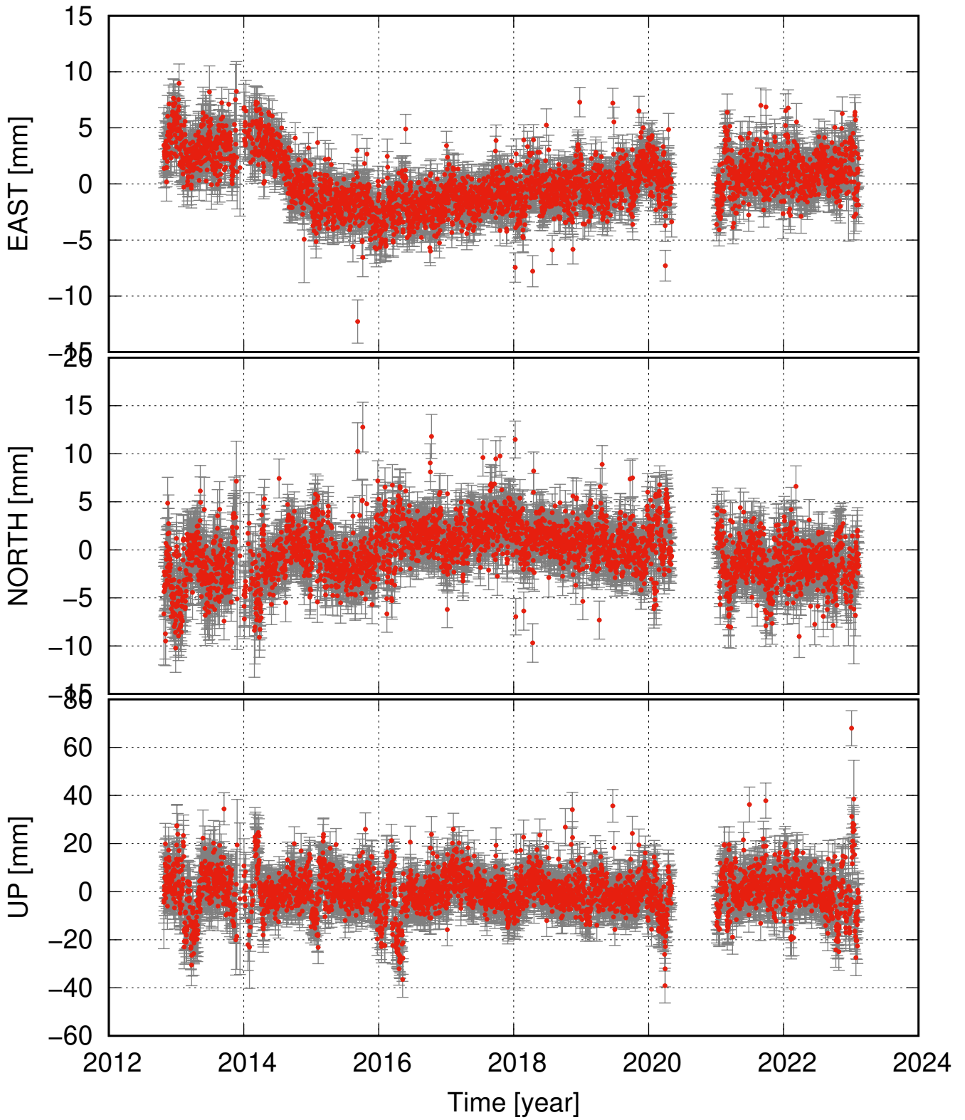
BJAC detrended and seasonal signal removed
