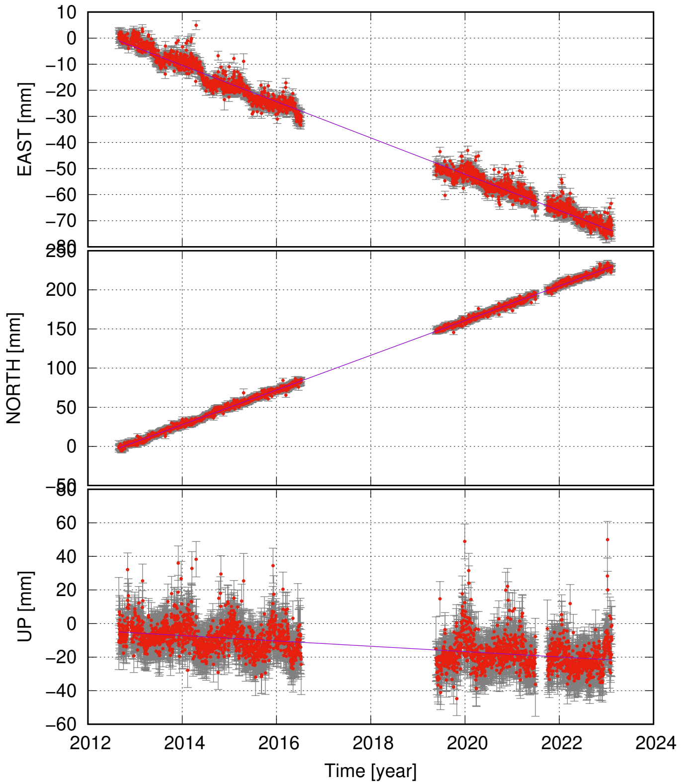
BAUG (66.04, -17.33) time series (ITRF 2014) v_e = -6.95 \pm 0.23 ; v_n = 22.17 \pm 0.19 ; v_u = -1.59 \pm 0.81 mm/yr
