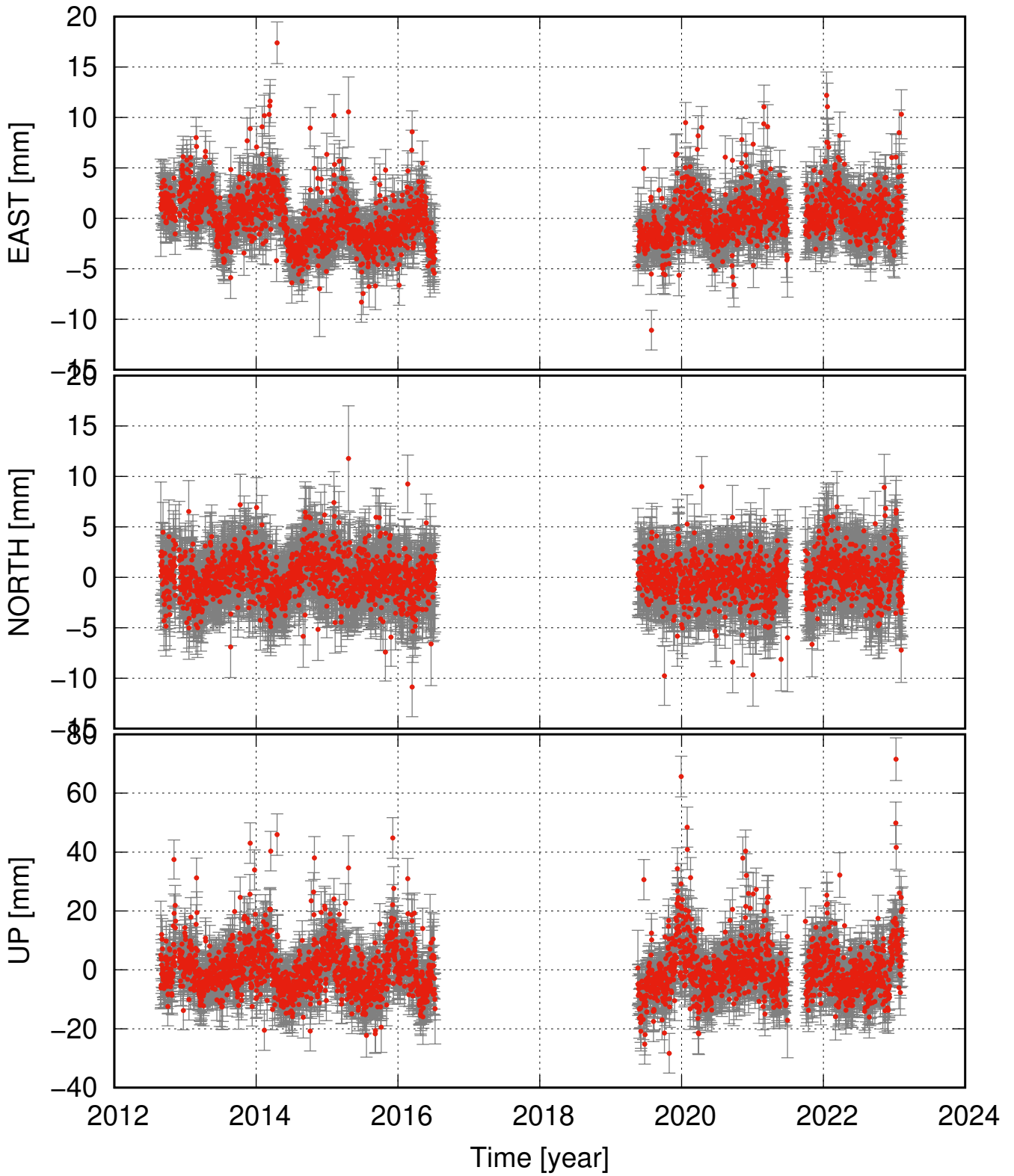
BAUG residual time series (some major events removed as well)
