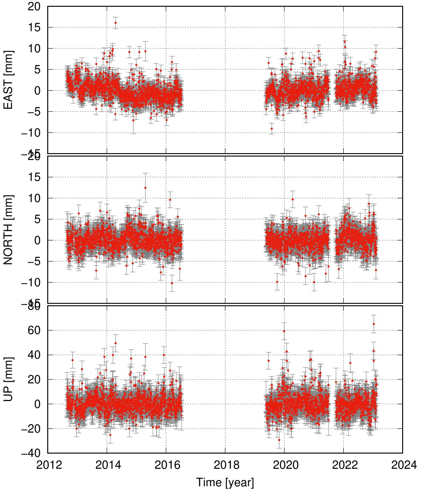
BAUG detrended and seasonal signal removed
