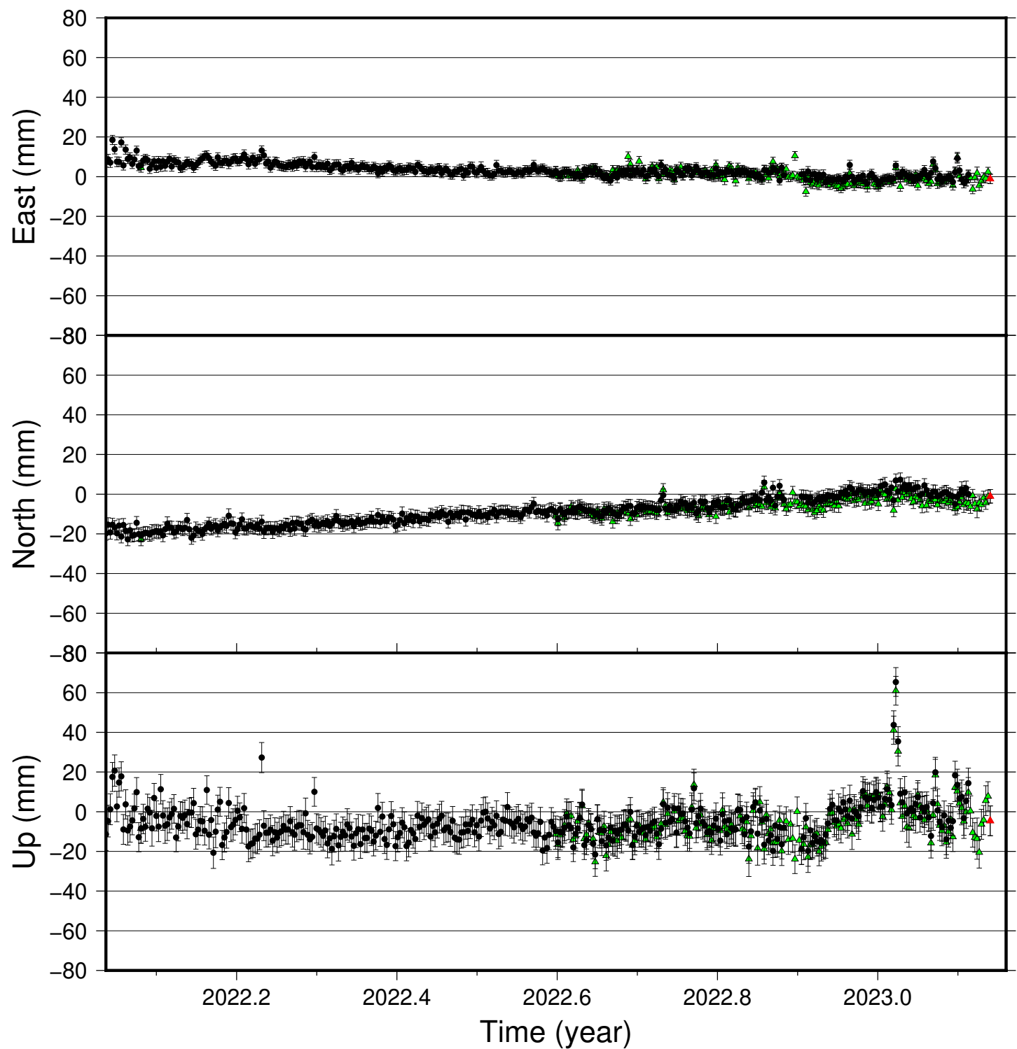
BAUG time series (IGS 2014), last 400 days
