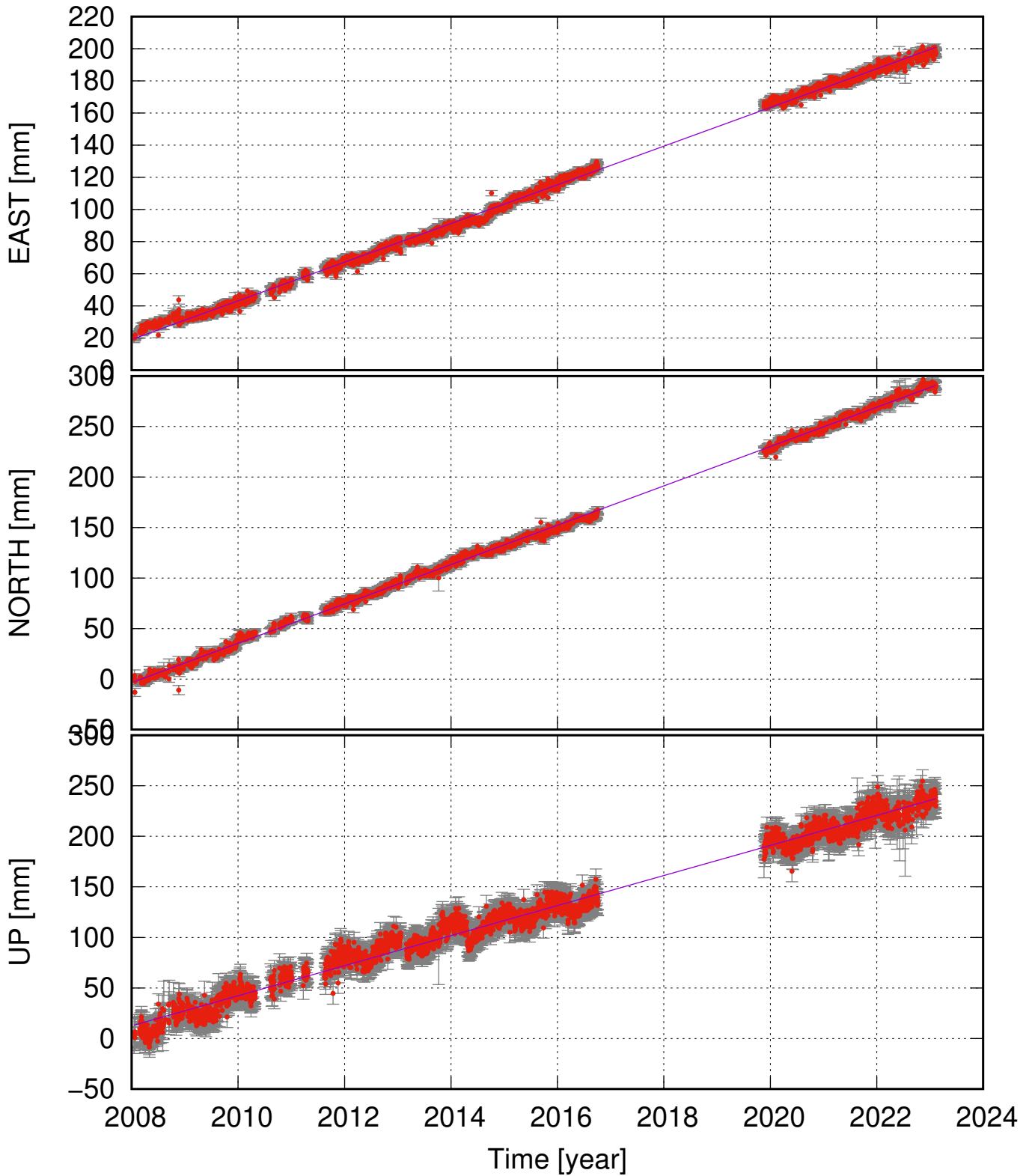
BALD (64.92, -15.75) time series (ITRF 2014) v_e = 12.03 \pm 0.15 ; v_n = 19.46 \pm 0.18 ; v_u = 14.86 \pm 0.55 mm/yr
