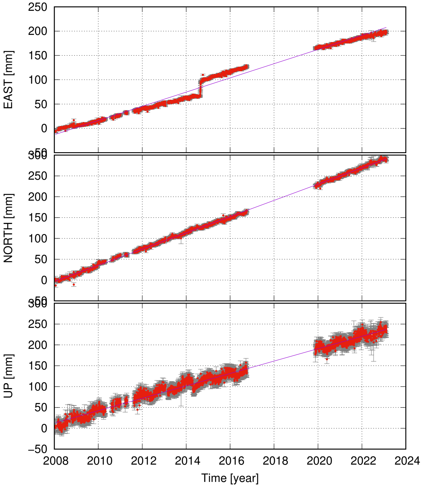
BALD (64.92, -15.75) time series (ITRF 2014) v_e = 14.60 \pm 0.57 ; v_n = 19.46 \pm 0.18 ; v_u = 14.86 \pm 0.55 mm/yr
