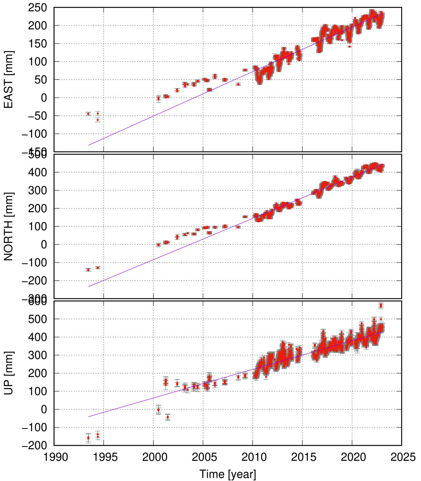
AUST (63.67, -19.08) time series (ITRF 2014) ve = 12.33 ± 0.54; vn = 22.87 ± 0.63; vu = 15.86 ± 0.86 mm/yr
