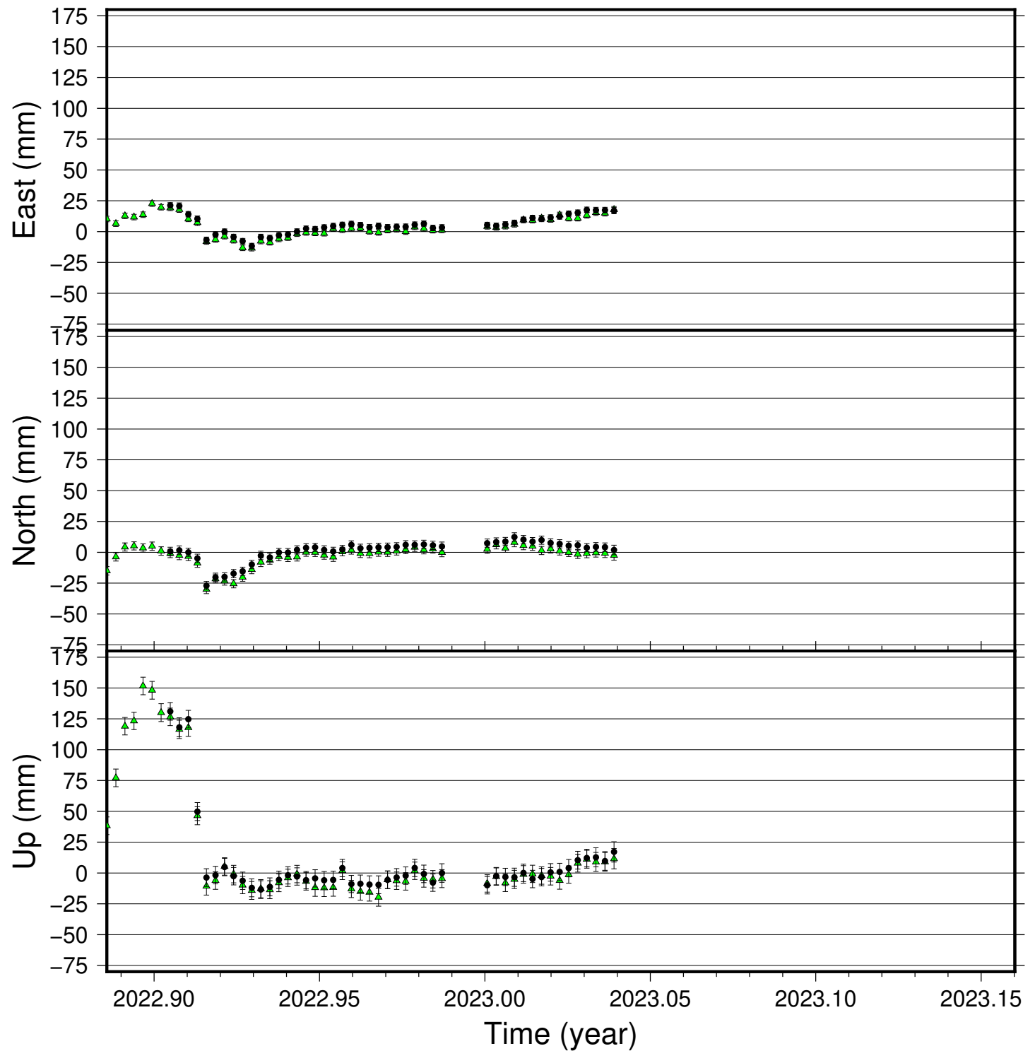
AUST time series (IGS 2014), last 100 days
