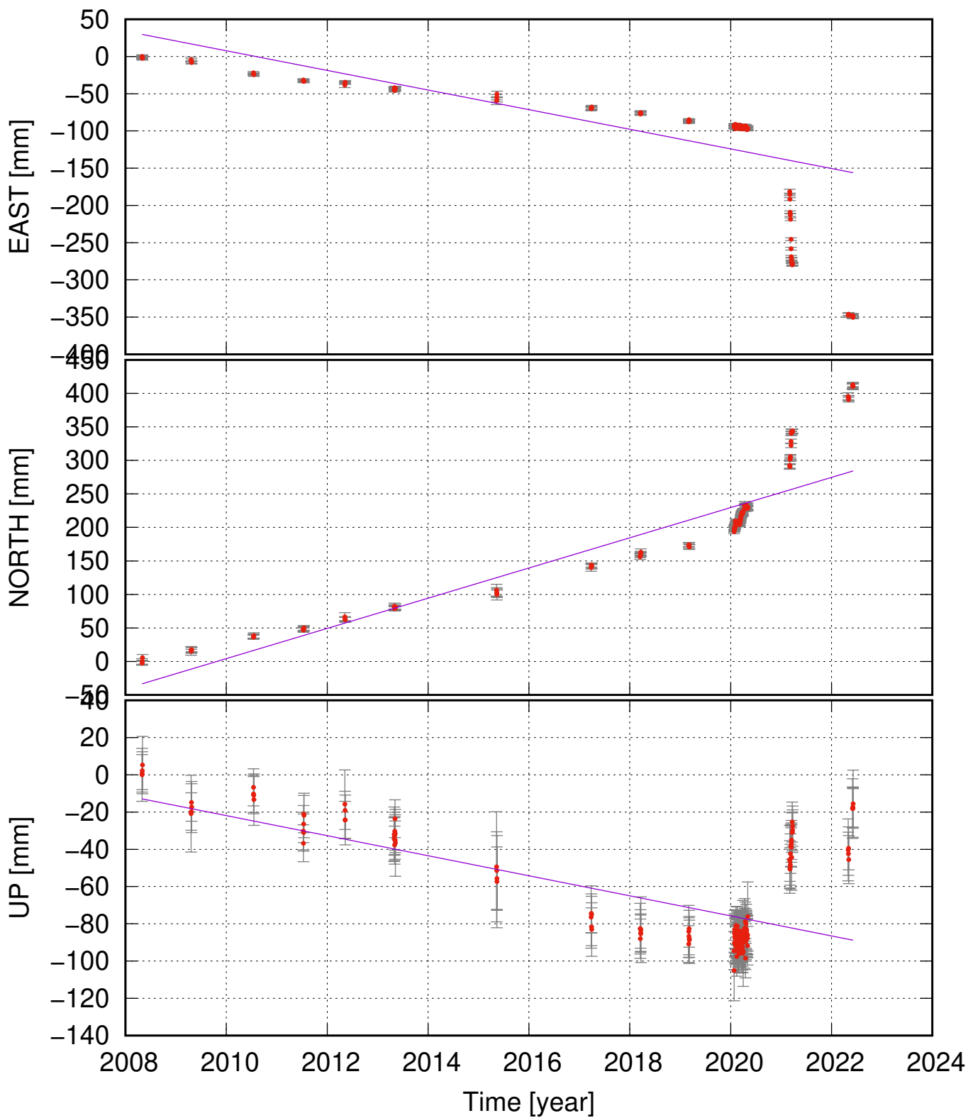
ARSE (63.91, -22.42) time series (ITRF 2014) v_e = -13.17 \pm 4.45 ; v_n = 22.54 \pm 2.93 ; v_u = -5.38 \pm 1.64 mm/yr
