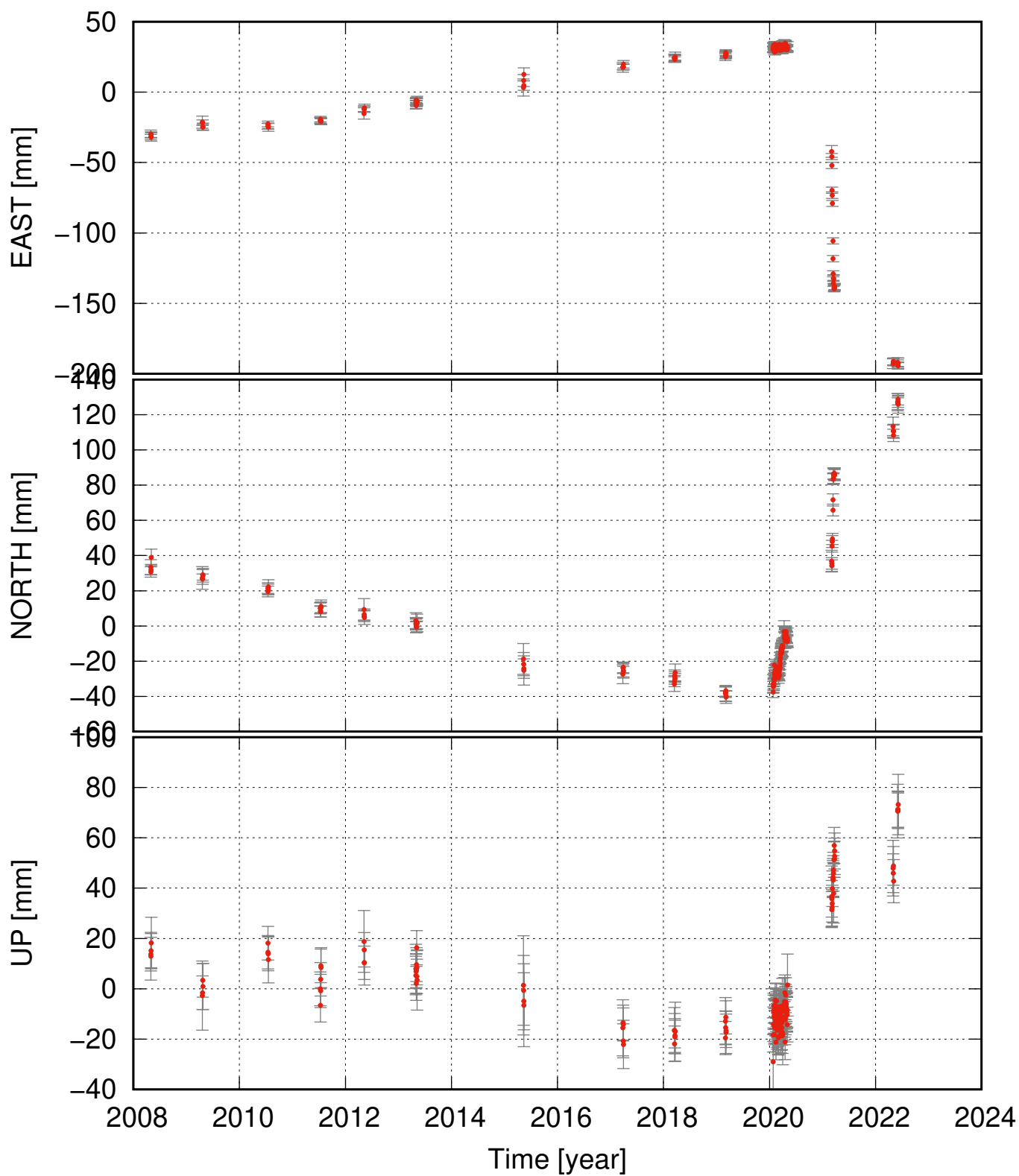
ARSE residual time series (some major events removed as well)
