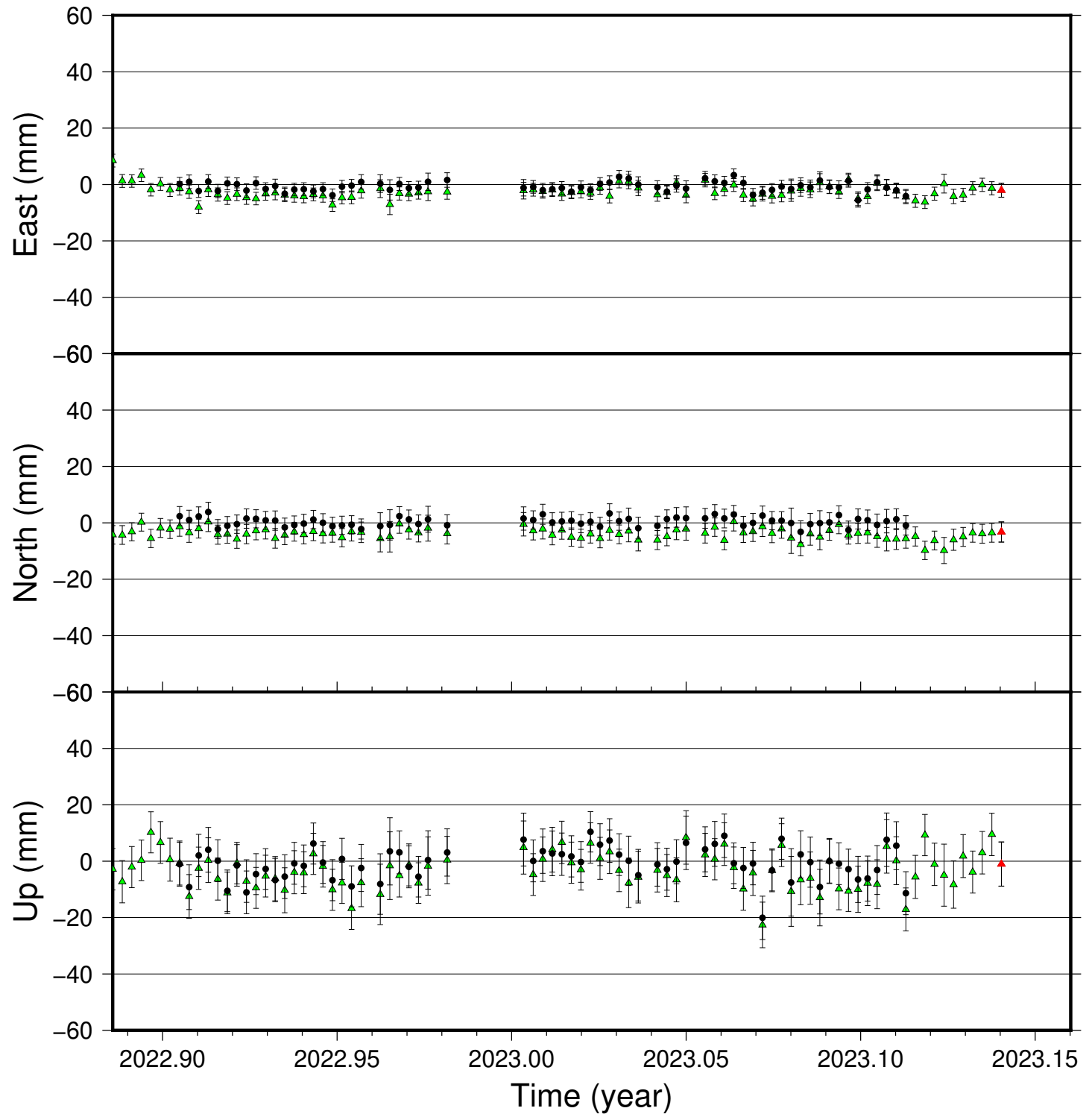
ARHO time series (IGS 2014), last 100 days
