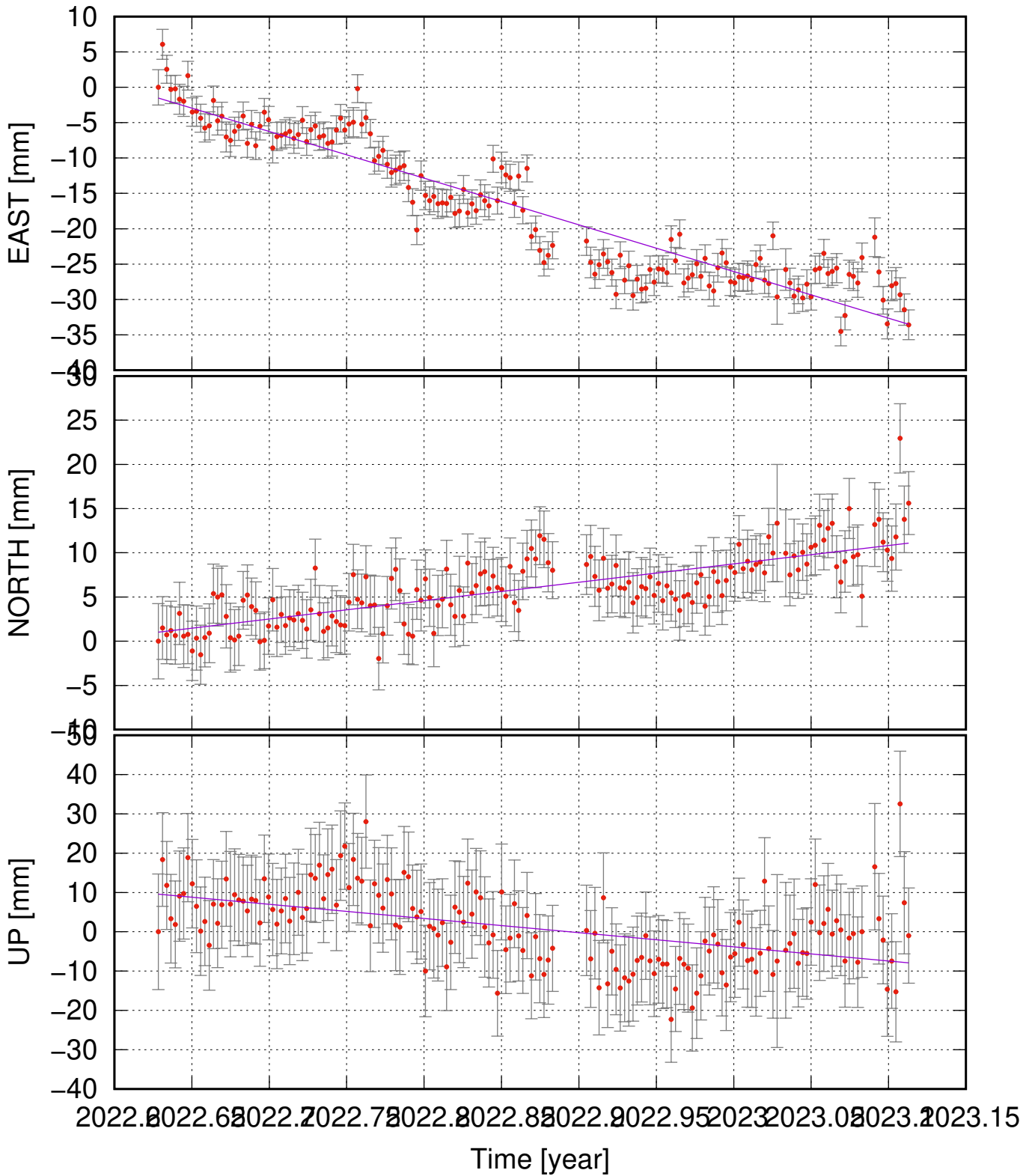
ALM2 (66.13, -19.07) time series (ITRF 2014) ve = -65.99 ± 7.23; vn = 20.76 ± 5.10; vu = -36.11 ± 17.05 mm/yr
