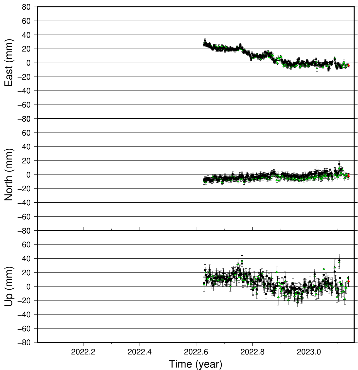
ALM2 time series (IGS 2014), last 400 days
