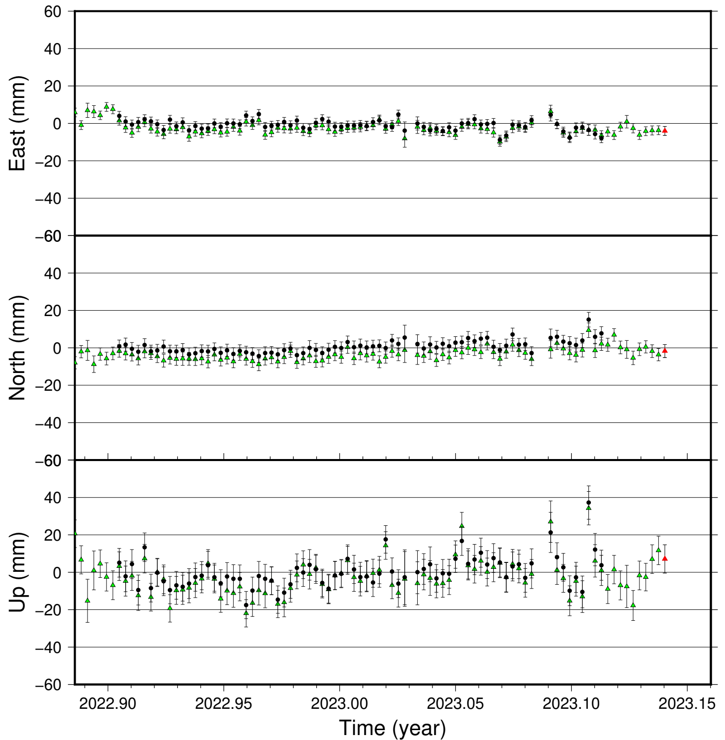
ALM2 time series (IGS 2014), last 100 days
