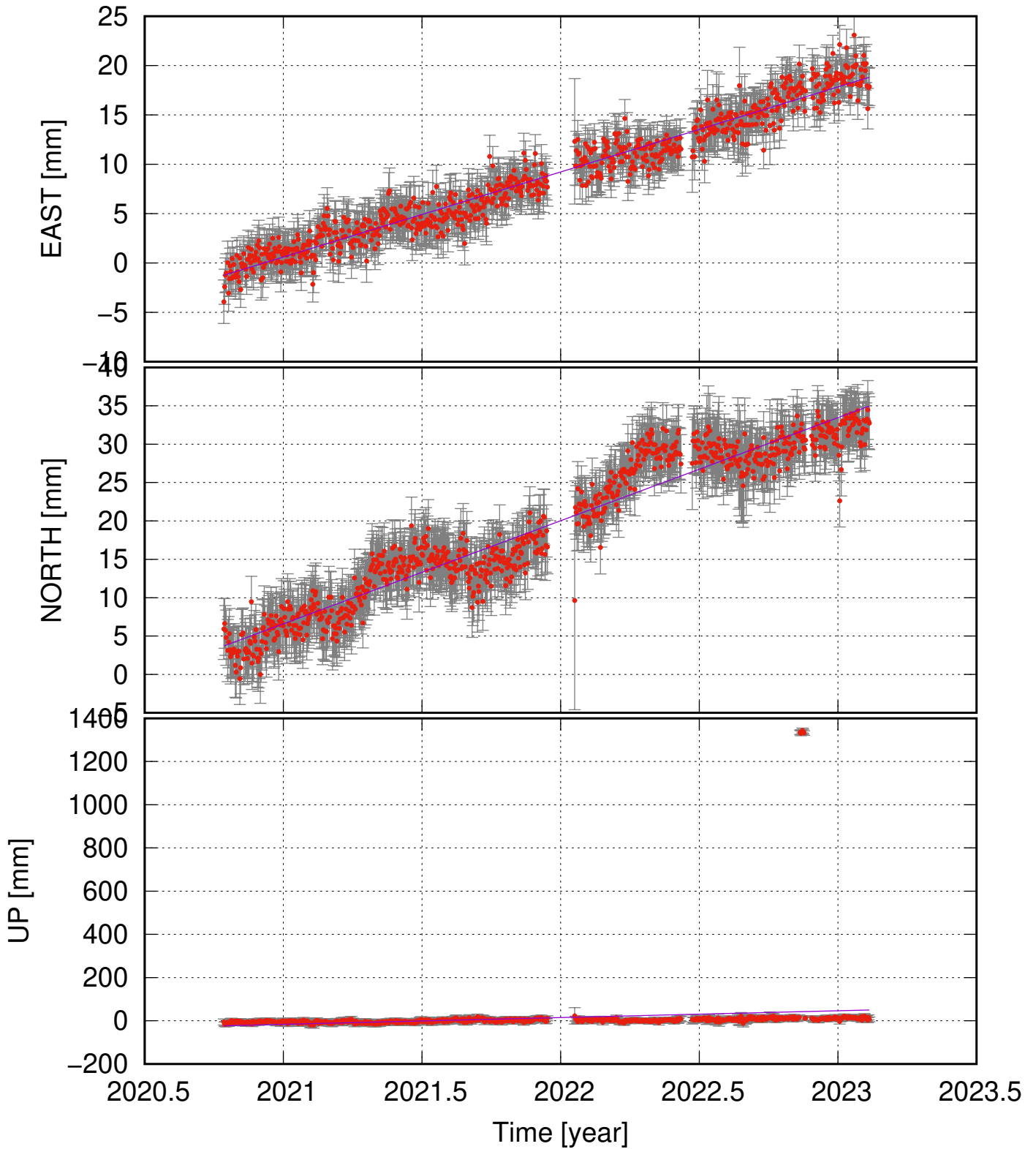
ALHV (63.45, -18.31) time series (ITRF 2014) v_e = 8.62 \pm 0.57 ; v_n = 13.43 \pm 1.13 ; v_u = 31.51 \pm 49.26 mm/yr
