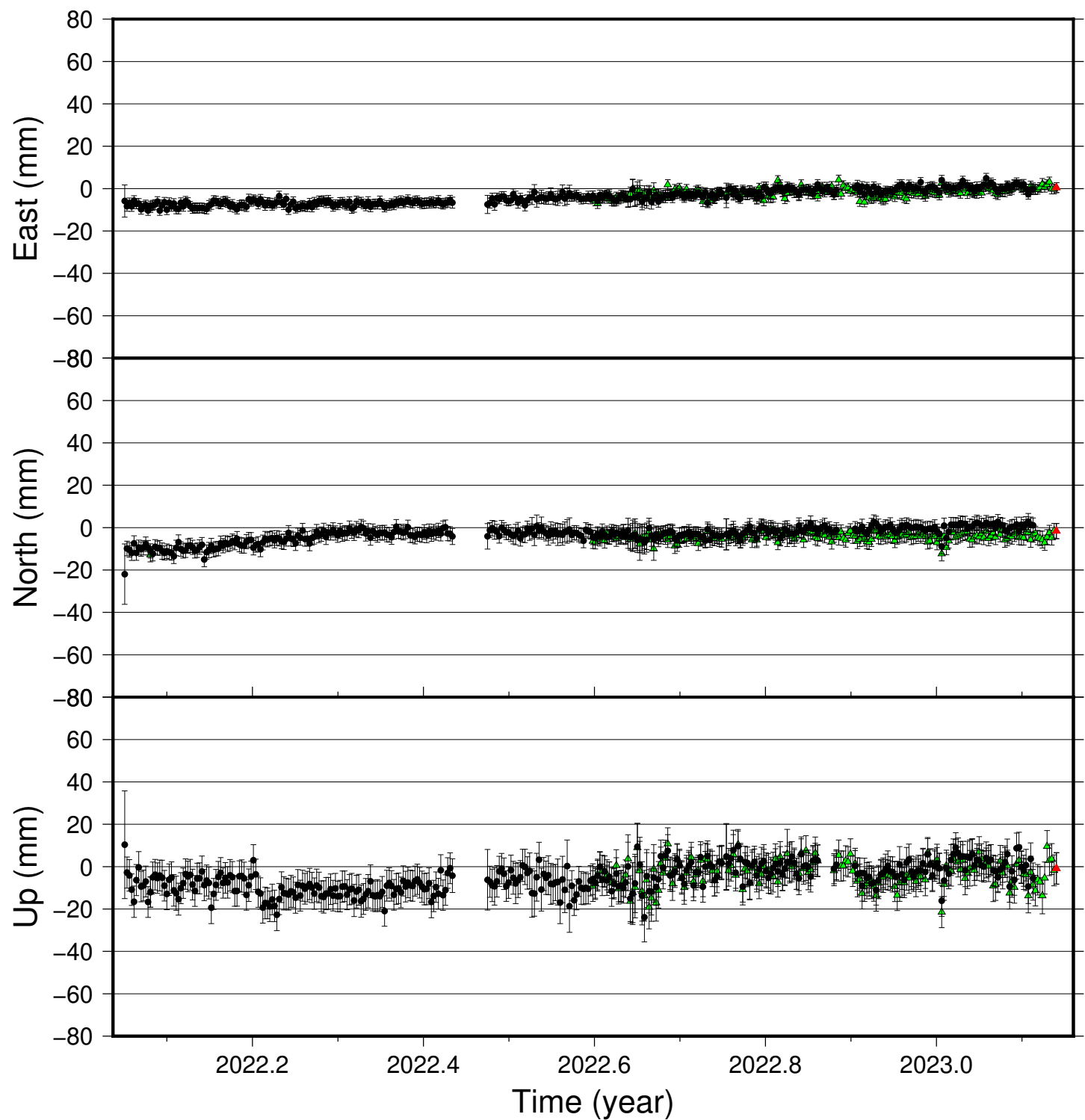
ALHV time series (IGS 2014), last 400 days
