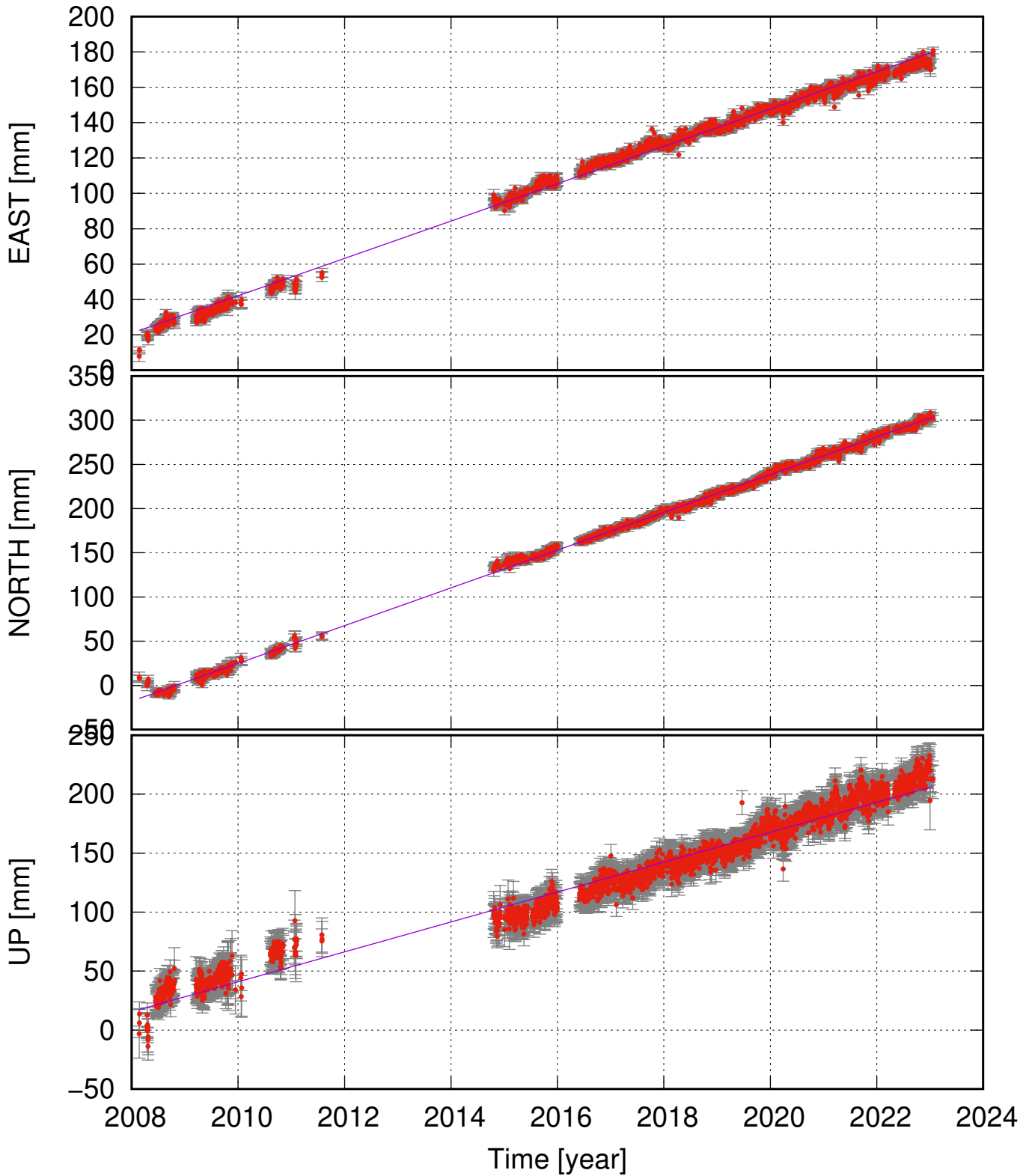
ALFD (64.98, -16.03) time series (ITRF 2014) v_e = 10.56 \pm 0.18 ; v_n = 21.34 \pm 0.20 ; v_u = 12.68 \pm 0.63 mm/yr
