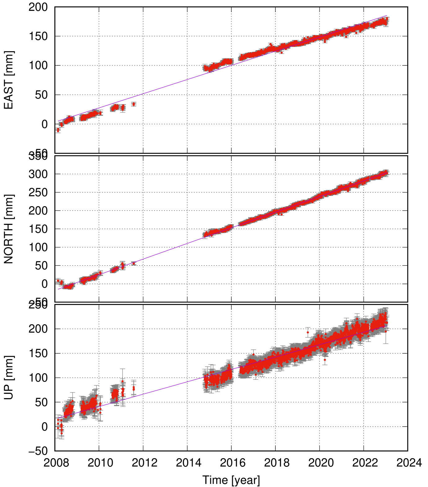
ALFD (64.98, -16.03) time series (ITRF 2014) ve = 12.09 ± 0.40; vn = 21.34 ± 0.20; vu = 12.68 ± 0.63 mm/yr
