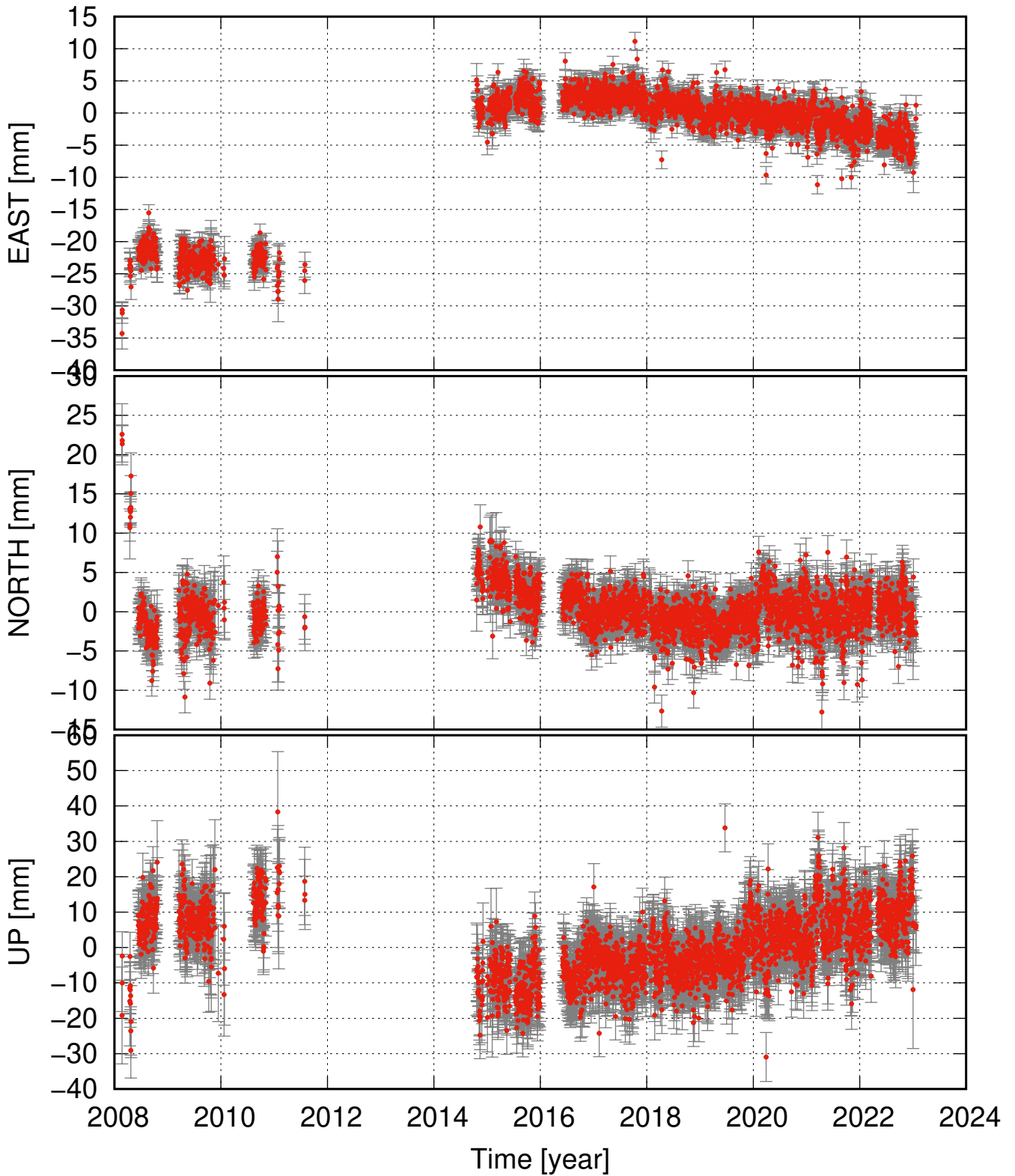
ALFD detrended and seasonal signal removed
