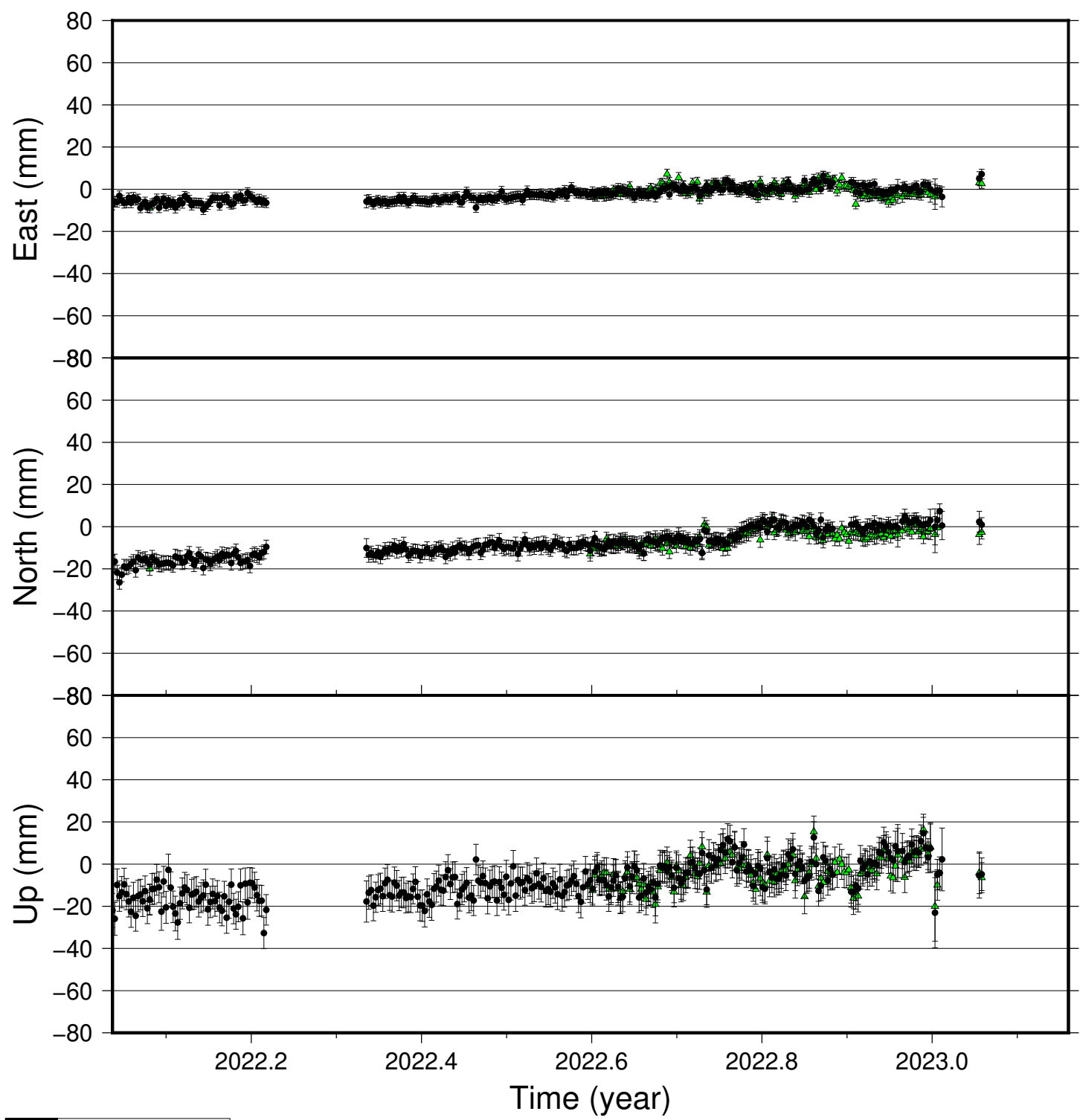
ALFD time series (IGS 2014), last 400 days
